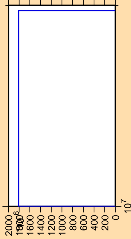
\Delta\sigma/\sigma vs. E for ^{193}\text{Os}(n,3n\alpha)
