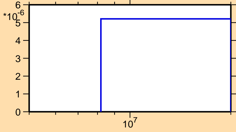
\sigma vs. E for ^{194}\text{Os}(n,d)
