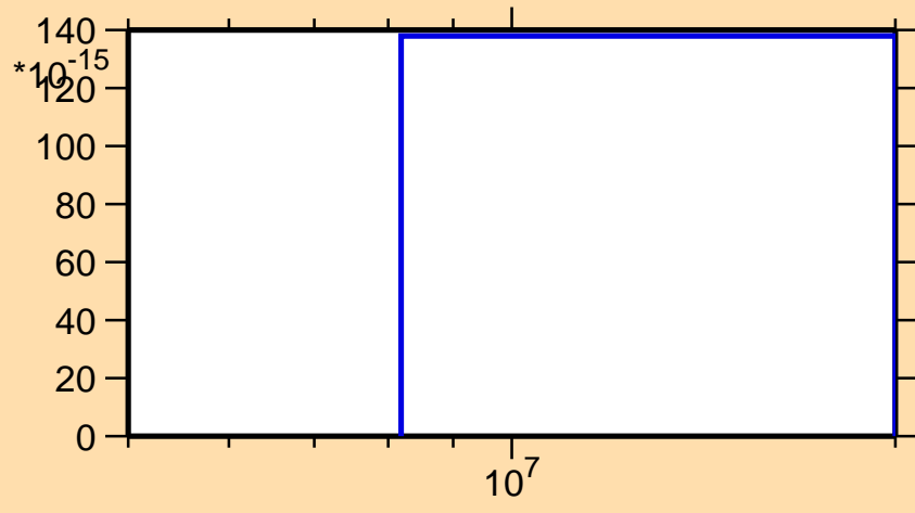
\sigma vs. E for ^{194}\text{Os}(n,2np)
