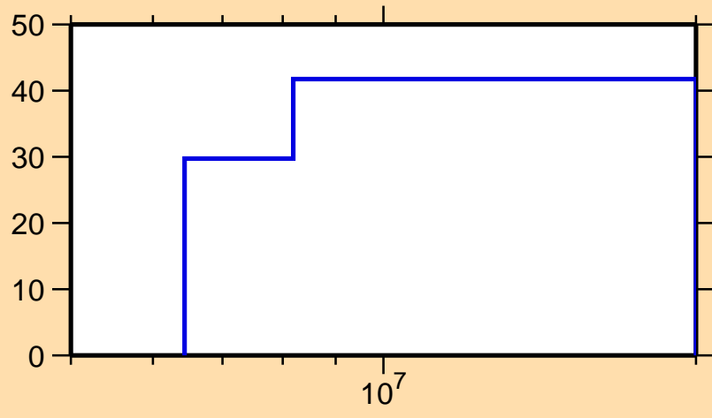
\Delta\sigma/\sigma vs. E for ^{194}\text{Os}(n,ncont.)
