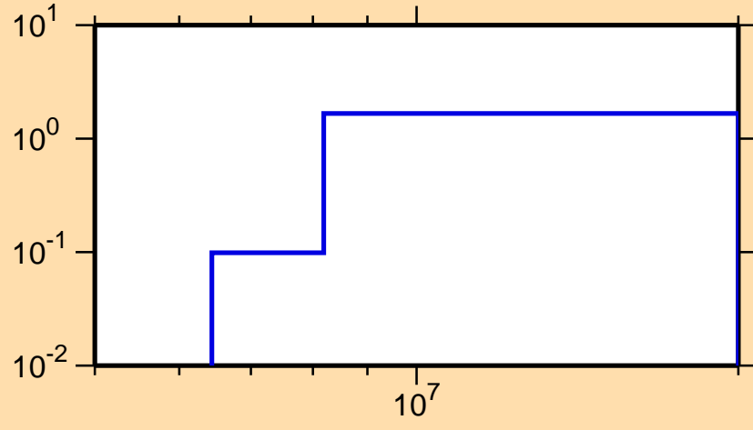
\sigma vs. E for ^{194}\text{Os}(n,2n)
