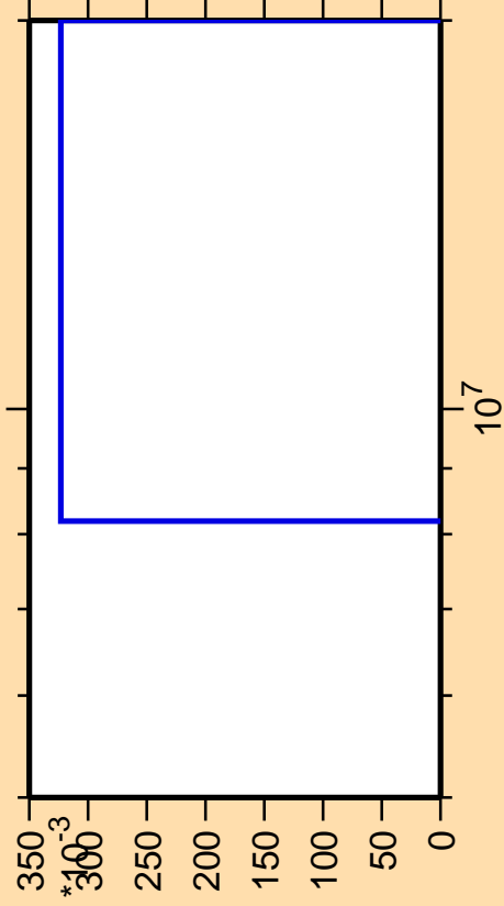
\Delta\sigma/\sigma vs. E for ^{194}\text{Os}(n,2np)
