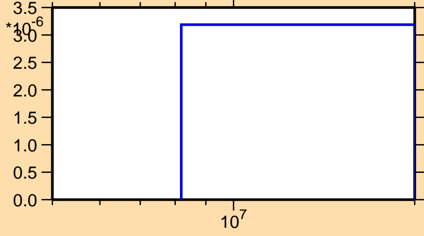
\sigma vs. E for ^{194}\text{Os}(n,np)
