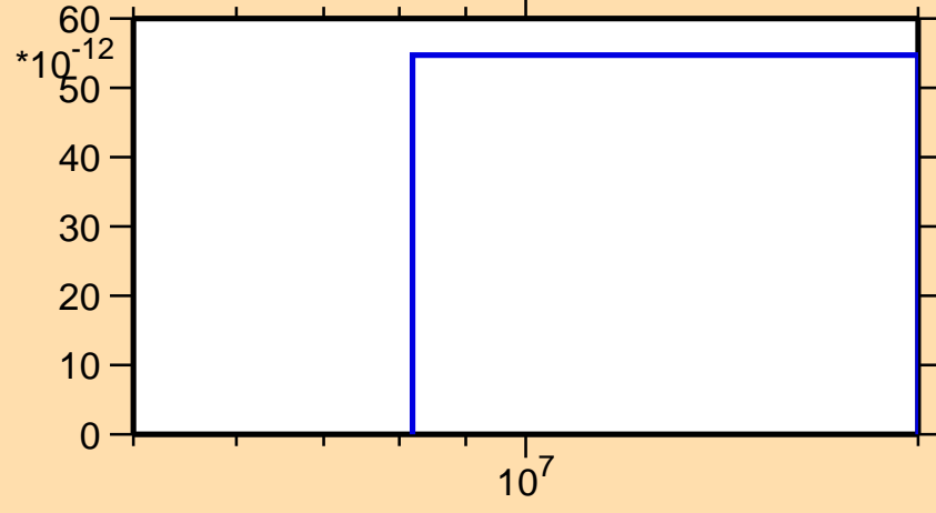
\sigma vs. E for ^{194}\text{Os}(n,2n\alpha)
