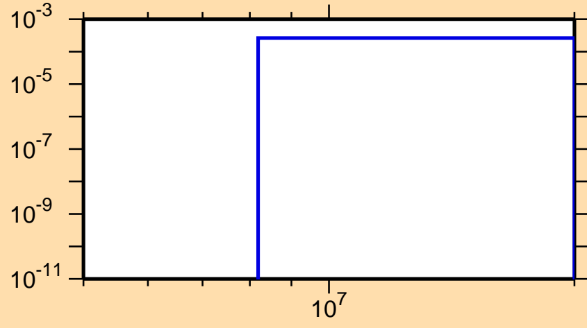
\sigma vs. E for ^{194}\text{Os}(n,p)
