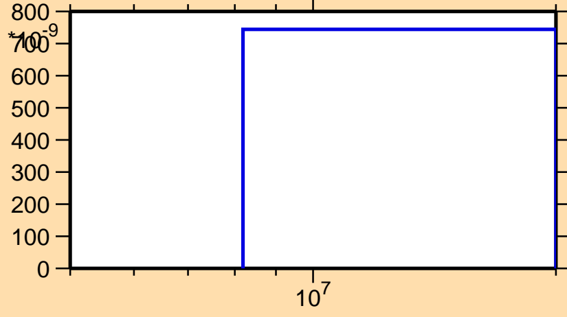
\sigma vs. E for ^{194}\text{Os}(n,t)
