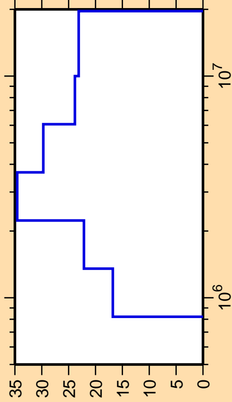
\Delta\sigma/\sigma vs. E for ^{195}\text{Os}(n,n_2)
