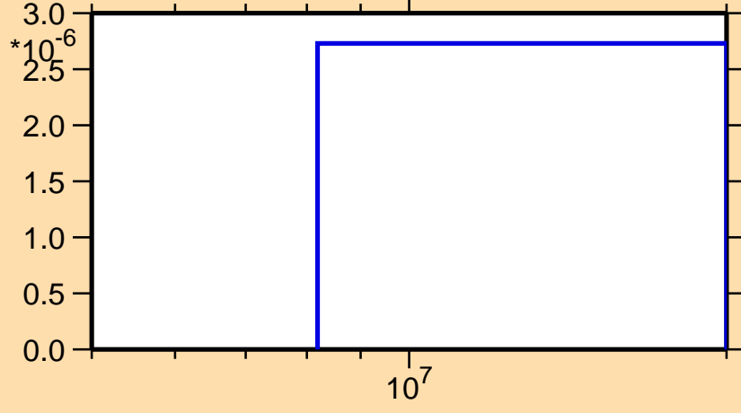
\sigma vs. E for ^{195}\text{Os}(n,t)
