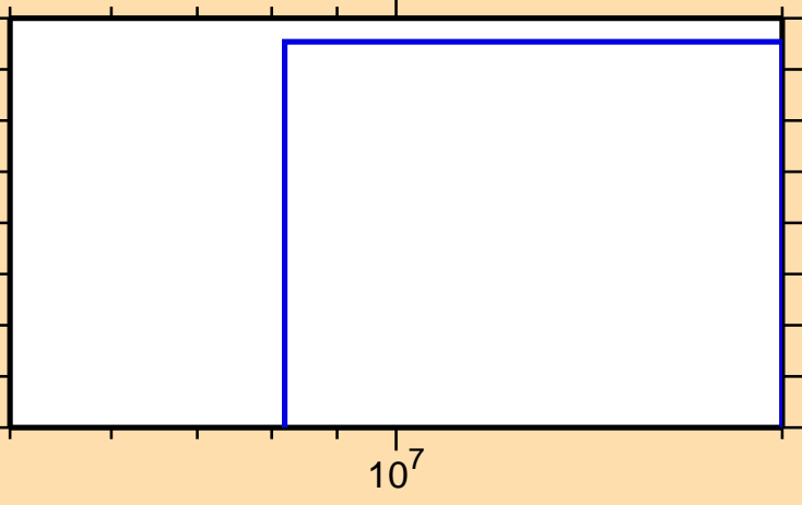
\sigma vs. E for ^{195}\text{Os}(n,d)
