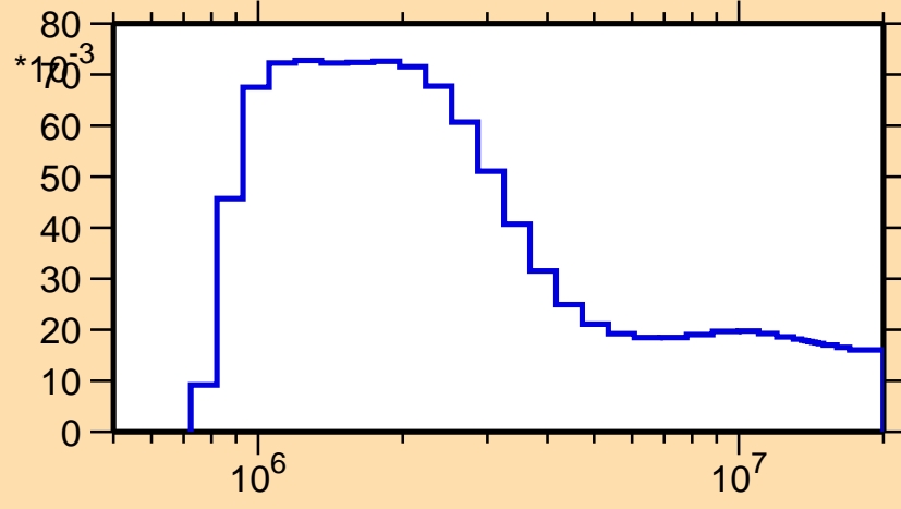
\sigma vs. E for ^{196}\text{Os}(n,n_3)
