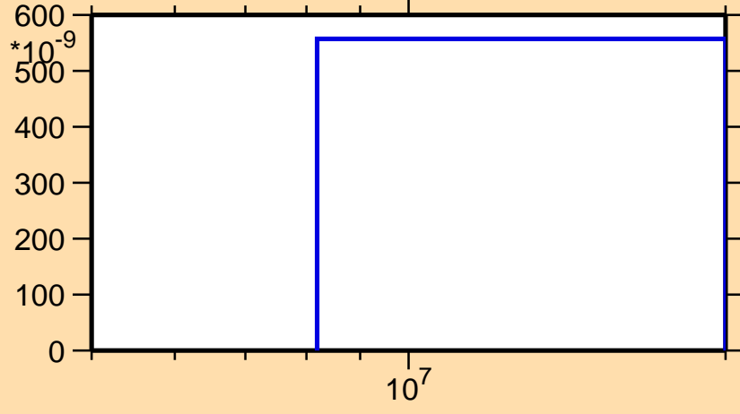
\sigma vs. E for ^{196}\text{Os}(n,t)
