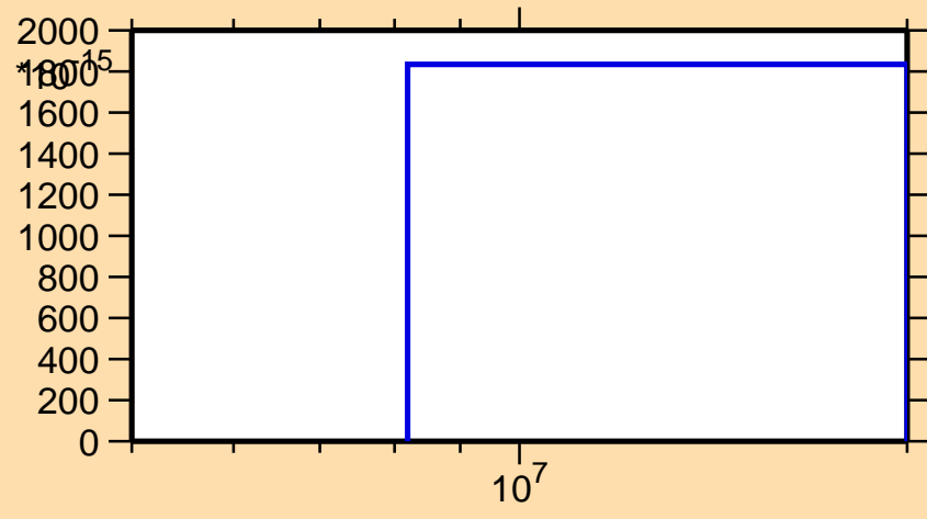
\sigma vs. E for ^{196}\text{Os}(n,nd)
