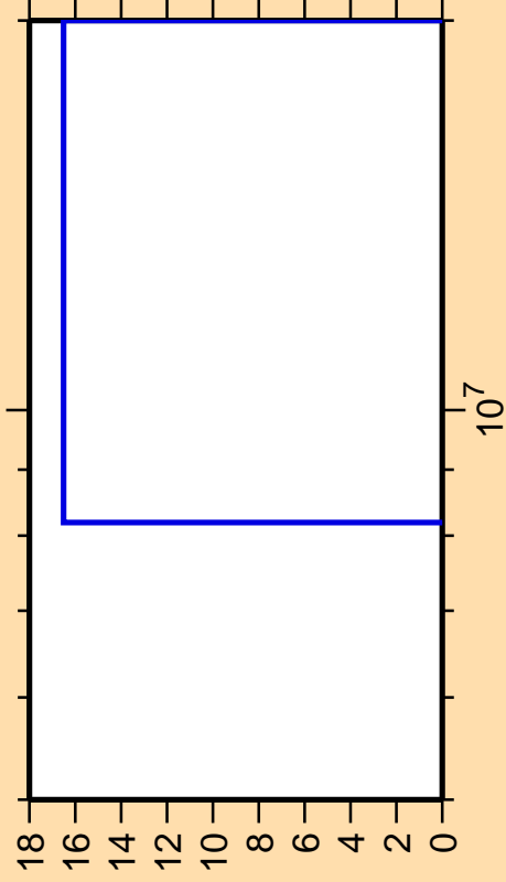
\Delta\sigma/\sigma vs. E for ^{196}\text{Os}(n,nd)
