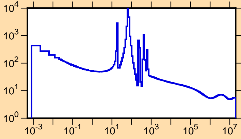
\sigma vs. E for ^{197}\text{Os}(n,\text{tot.})
