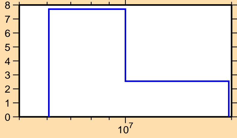
\Delta\sigma/\sigma vs. E for ^{197}\text{Os}(n,\text{tot.})
