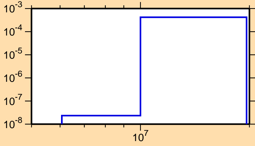
\sigma vs. E for ^{197}\text{Os}(n,p)
