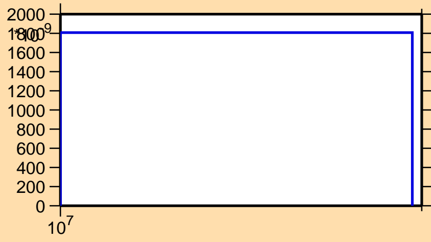
\sigma vs. E for ^{197}\text{Os}(n,np)
