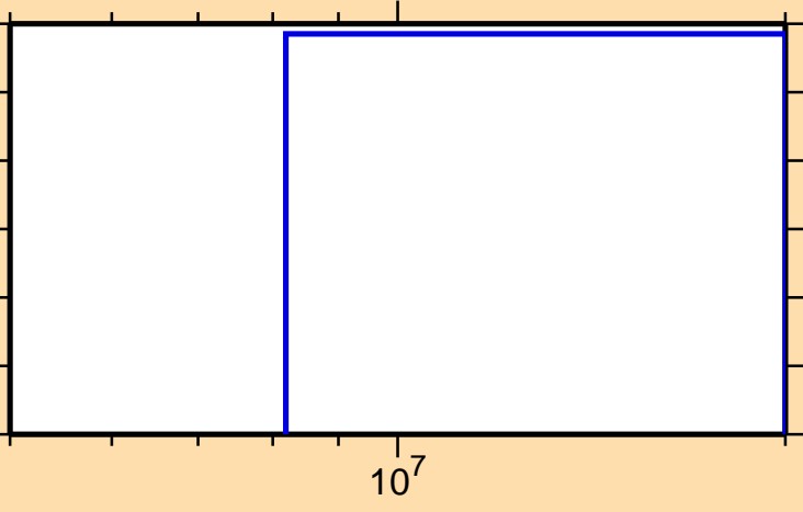
\sigma vs. E for ^{197}\text{Os}(n,3n)
