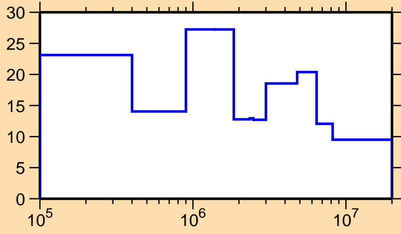
\Delta\sigma/\sigma vs. E for ^{197}\text{Os}(n, el.)
