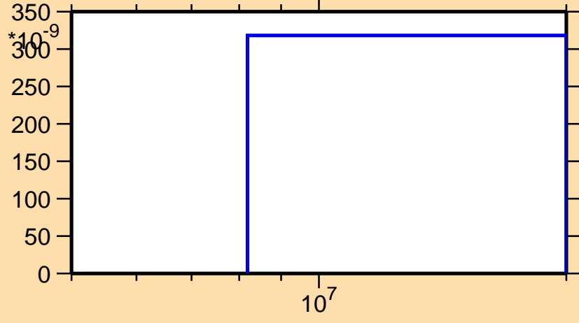
\sigma vs. E for ^{198}\text{Os}(n,t)
