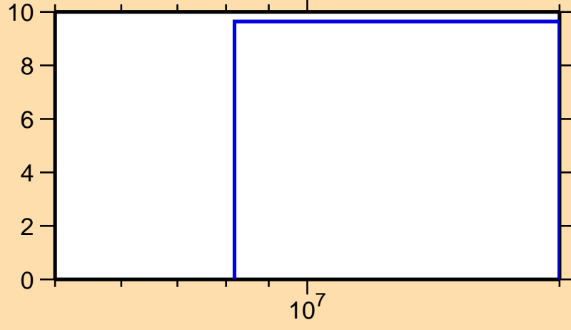
\Delta\sigma/\sigma vs. E for ^{198}\text{Os}(n,el.)
