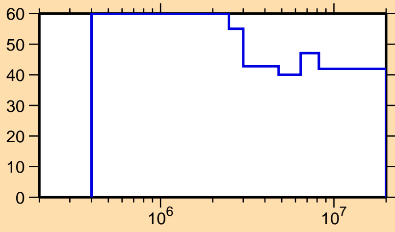
\Delta\sigma/\sigma vs. E for ^{198}\text{Os}(n,n_1)
