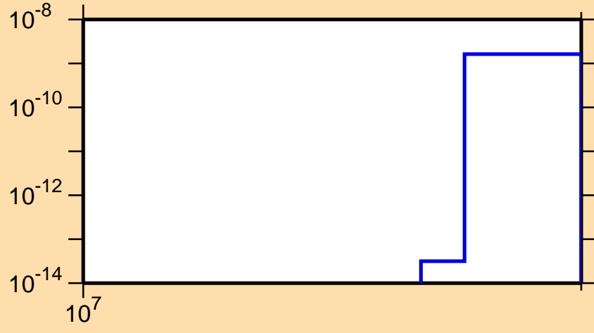
\sigma vs. E for ^{200}\text{Os}(n,nt)
