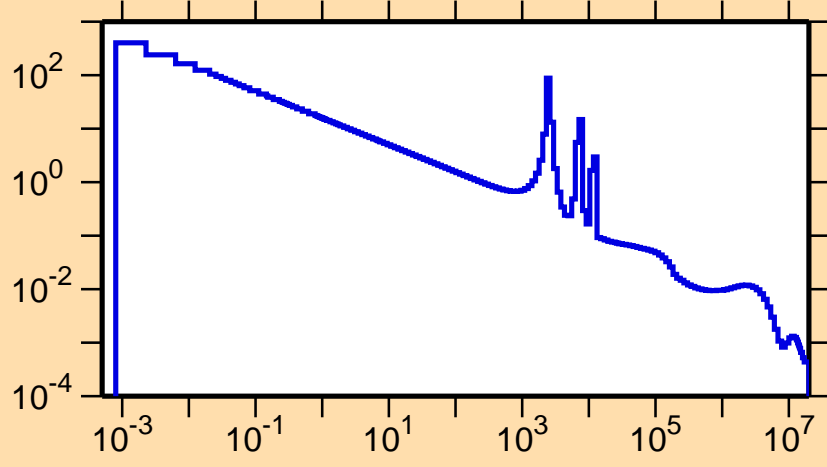
\sigma vs. E for ^{200}\text{Os}(n,\gamma)
