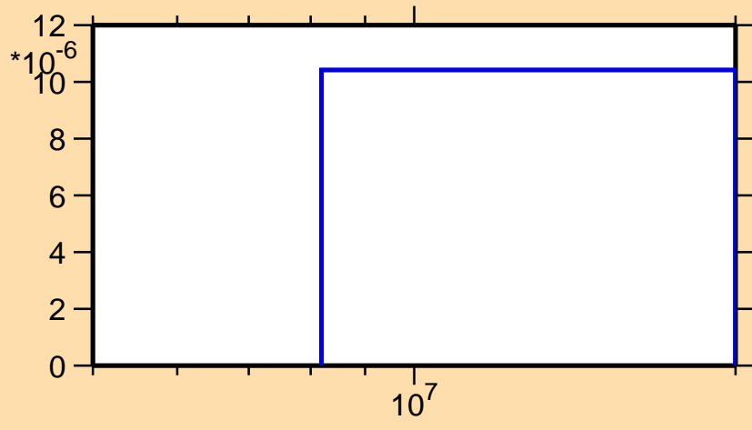
\sigma vs. E for ^{200}\text{Os}(n,p)
