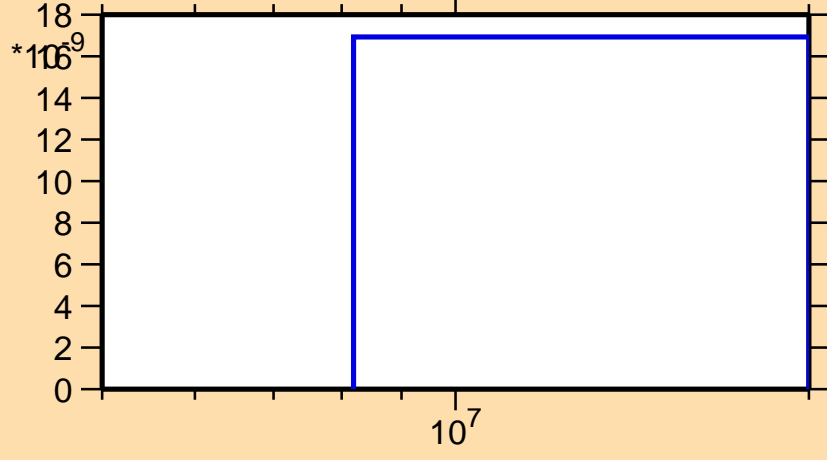
\sigma vs. E for ^{200}\text{Os}(n,n\alpha)
