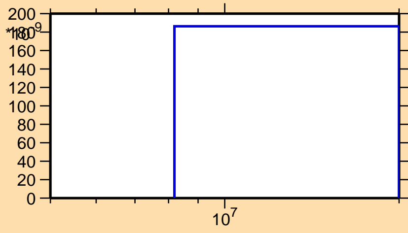
\sigma vs. E for ^{200}\text{Os}(n,t)
