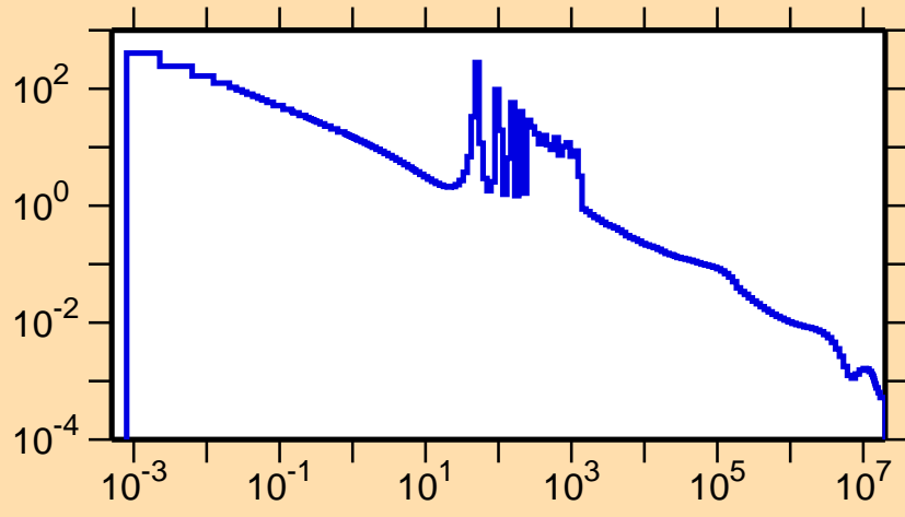
\sigma vs. E for ^{201}\text{Os}(n,\gamma)
