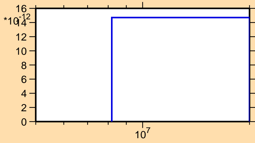
\sigma vs. E for ^{201}\text{Os}(n,\text{nd})
