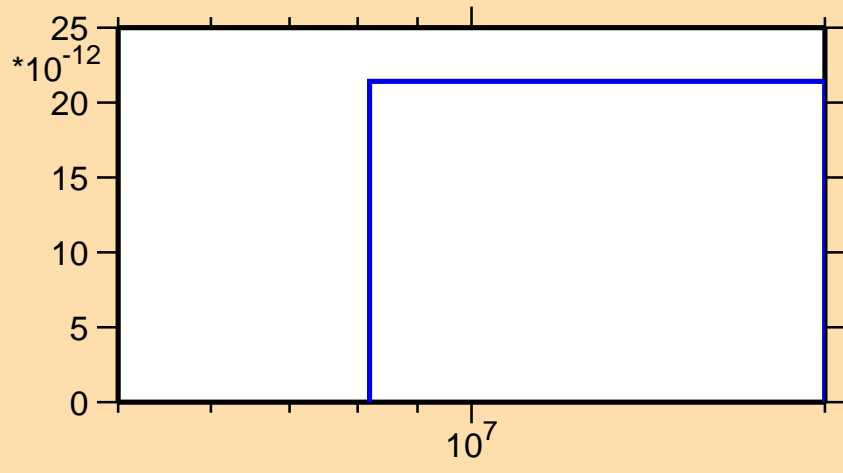
\sigma vs. E for ^{201}\text{Os}(n,nt)
