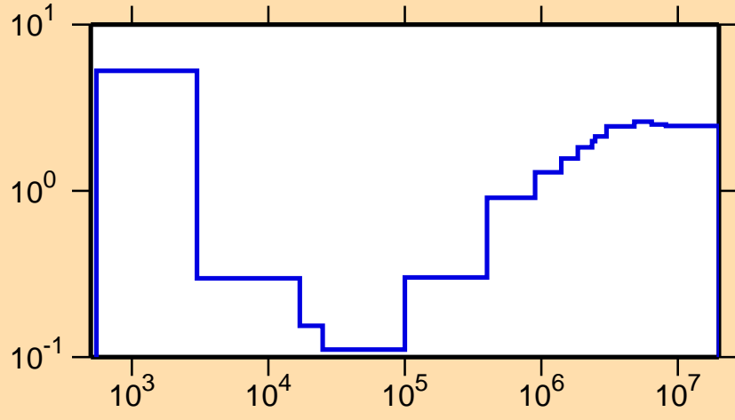
\sigma vs. E for ^{201}\text{Os}(n,\text{nonel.})
