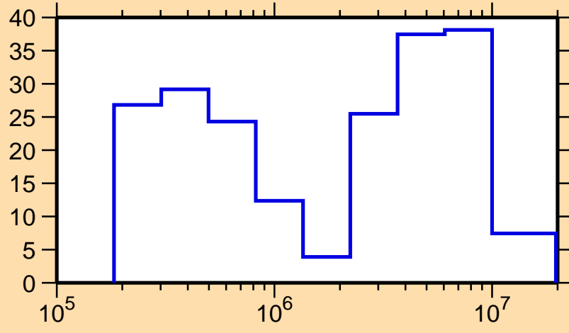
\Delta\sigma/\sigma vs. E for ^{29}\text{P}(n,el.)
