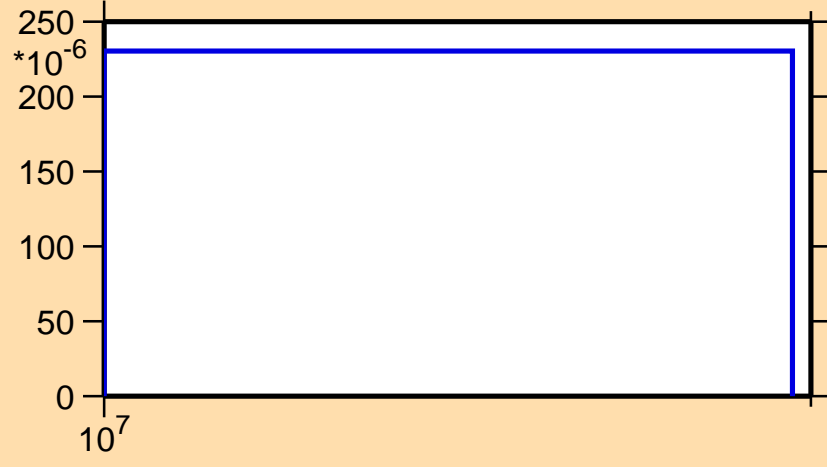
\sigma vs. E for ^{29}\text{P}(n,\text{pd})
