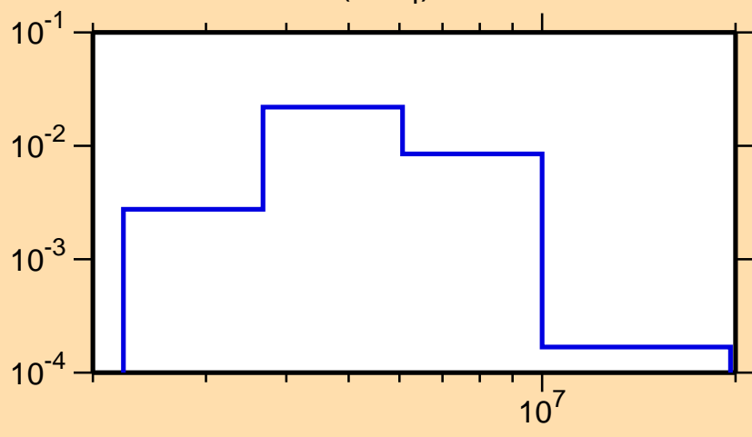
\sigma vs. E for ^{29}\text{P}(n,n_4)
