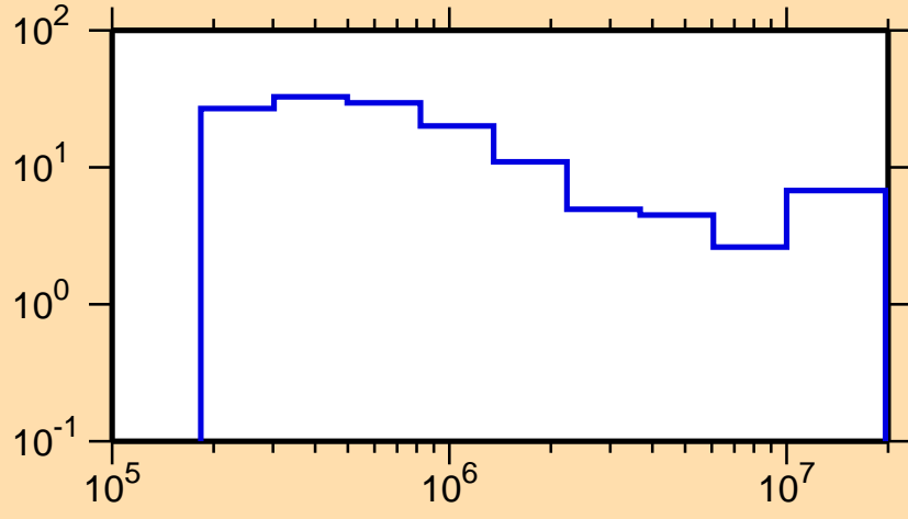
\Delta\sigma/\sigma vs. E for ^{29}\text{P}(n,\text{nonel.})
