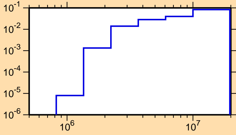
\sigma vs. E for ^{29}\text{P}(n,d)
