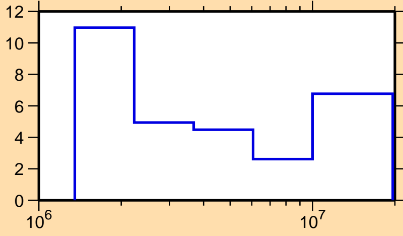
\Delta\sigma/\sigma vs. E for ^{29}\text{P}(n,\text{nonel.})
