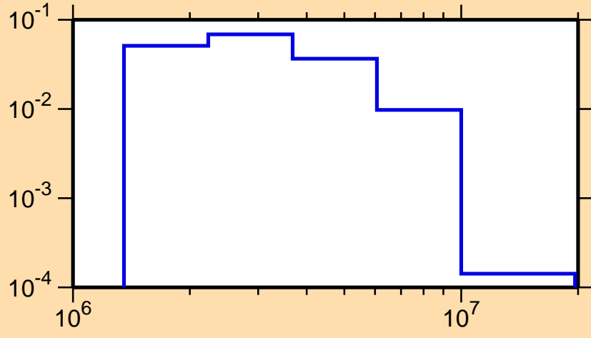
\sigma vs. E for ^{29}\text{P}(n,n_1)
