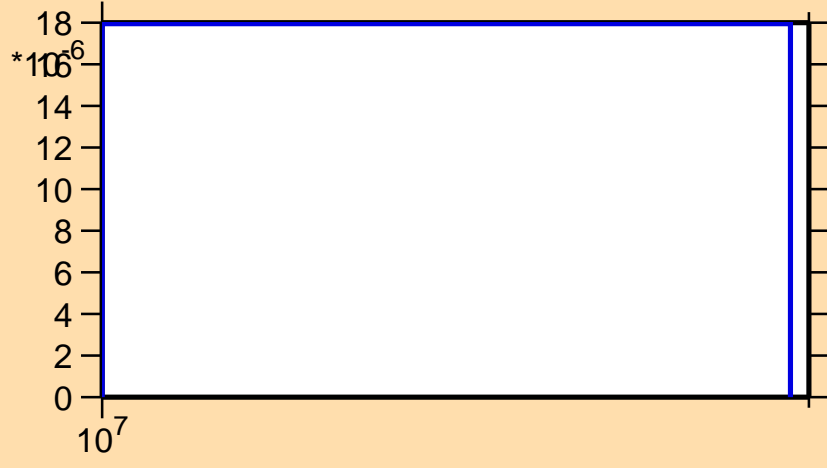
\sigma vs. E for ^{29}\text{P}(n,t)
