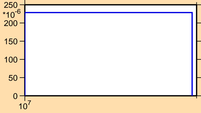
\sigma vs. E for ^{29}\text{P}(n,n\alpha)
