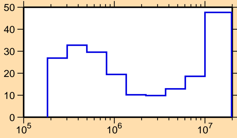
\Delta\sigma/\sigma vs. E for ^{29}\text{P}(n,p)
