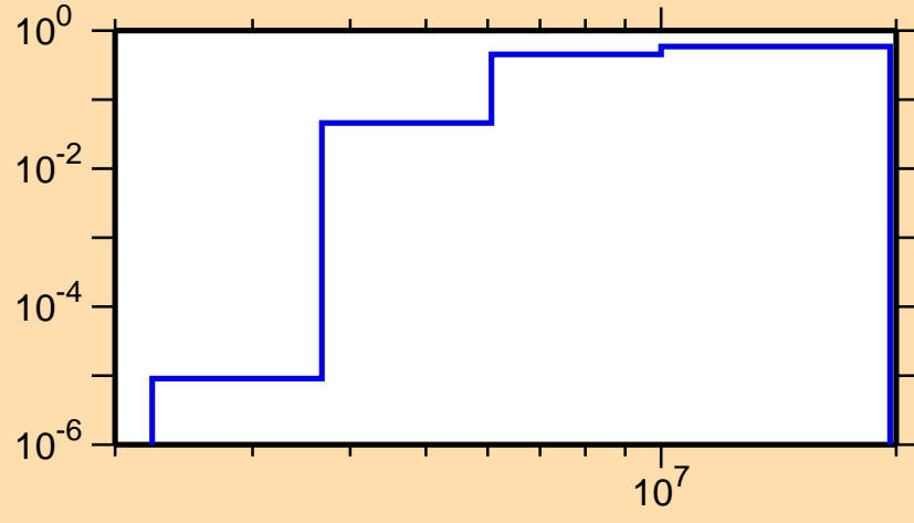
\sigma vs. E for ^{29}\text{P}(n,np)
