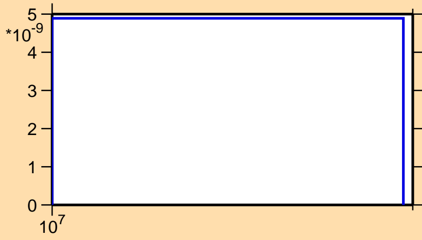
\sigma vs. E for ^{29}\text{P}(n,2n)
