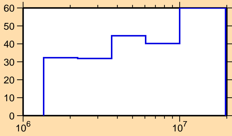
\Delta\sigma/\sigma vs. E for ^{29}\text{P}(n,n_1)
