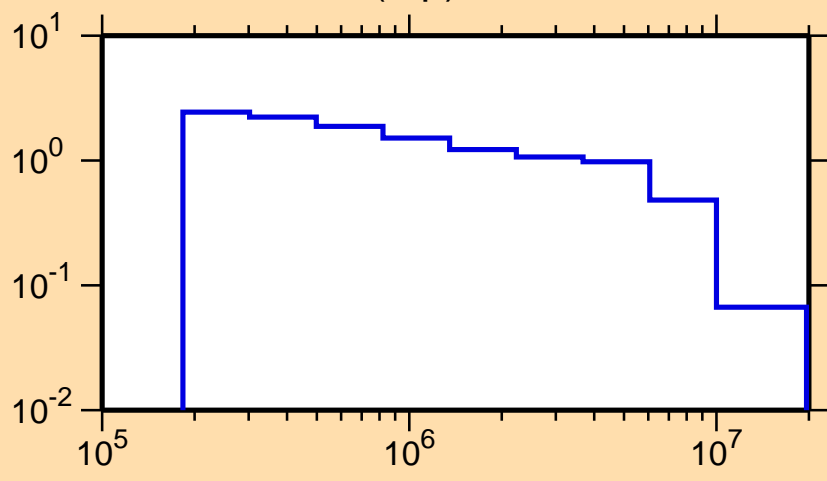
\sigma vs. E for ^{29}\text{P}(n,p)
