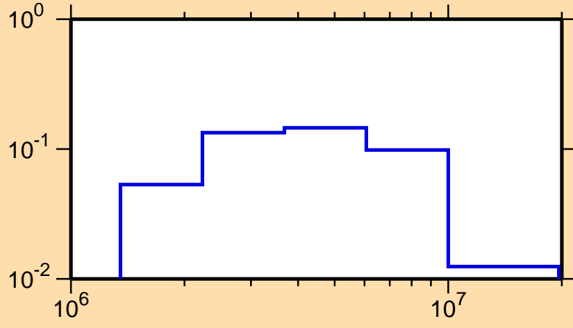
\sigma vs. E for ^{29}\text{P}(n,\text{inel.})
