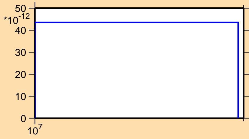
\sigma vs. E for ^{29}\text{P}(n,nd)
