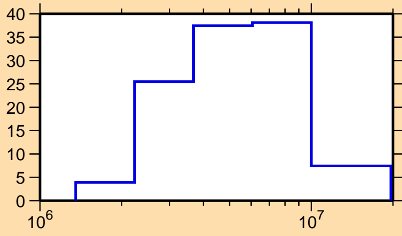
\Delta\sigma/\sigma vs. E for ^{29}\text{P}(n,\text{el.})
