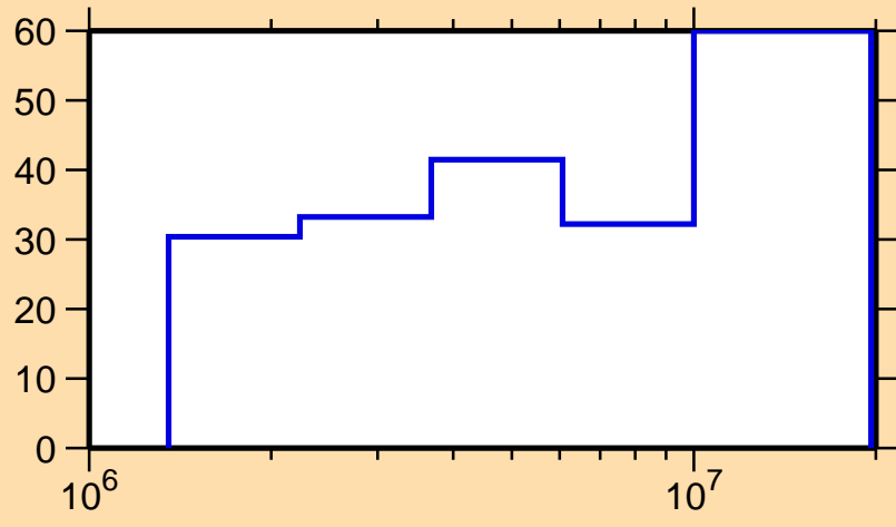
\Delta\sigma/\sigma vs. E for ^{29}\text{P}(n,\text{inel.})
