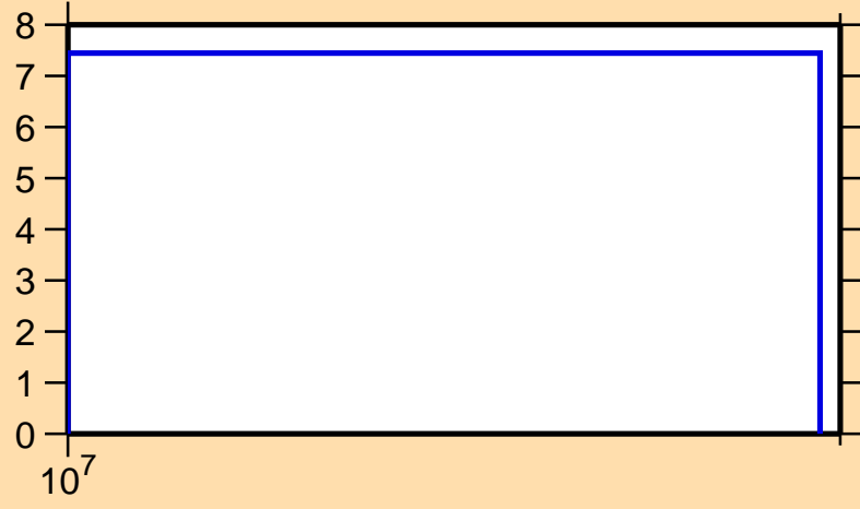
\Delta\sigma/\sigma vs. E for ^{29}\text{P}(n,\text{el.})
