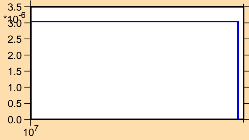
\sigma vs. E for ^{29}\text{P} (mt 45)
