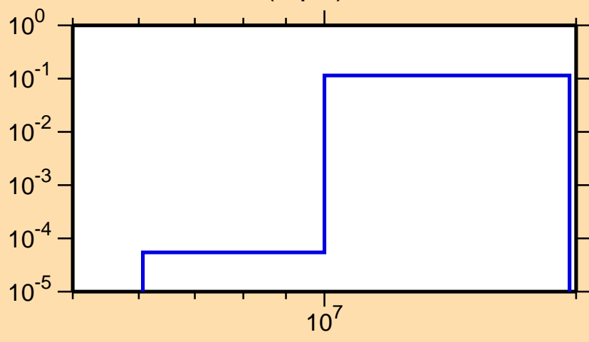
\sigma vs. E for ^{29}\text{P}(n,p\alpha)
