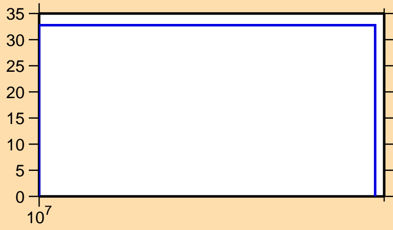
\Delta\sigma/\sigma vs. E for ^{29}\text{P}(n,2n)
