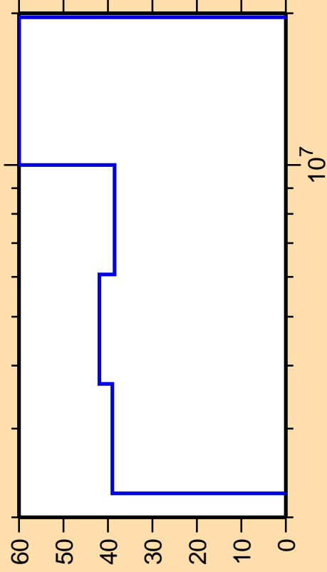
\Delta\sigma/\sigma vs. E for ^{29}\text{P}(n,n_4)
