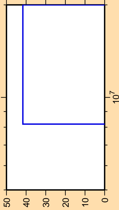
\Delta\sigma/\sigma vs. E for ^{29}\text{P}(n,p)
