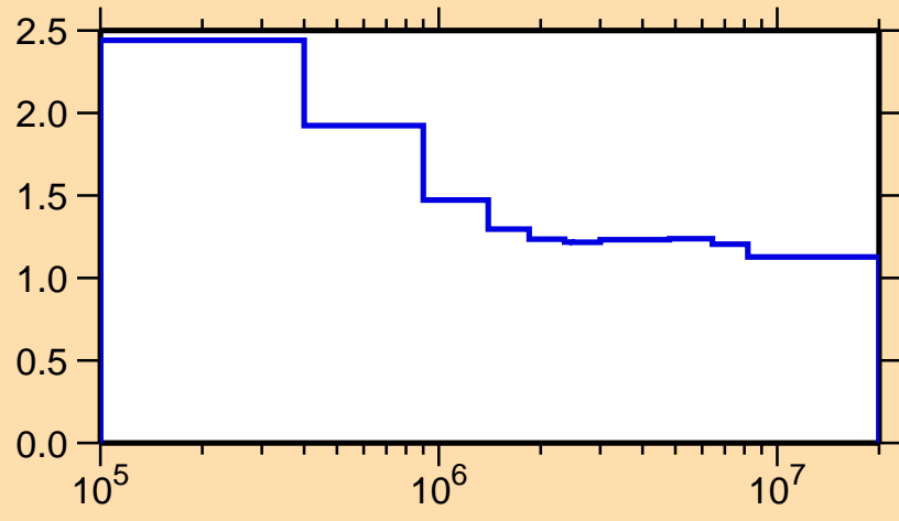
\sigma vs. E for ^{29}\text{P}(n,\text{nonel.})
