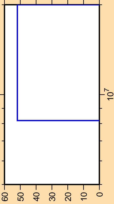
\Delta\sigma/\sigma vs. E for ^{29}\text{P}(n,t)
