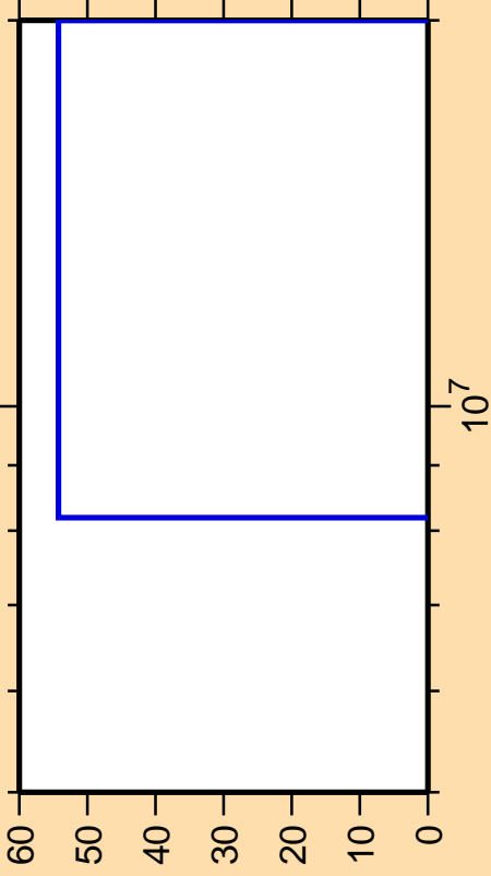
\Delta\sigma/\sigma vs. E for ^{29}\text{P} (mt 45)
