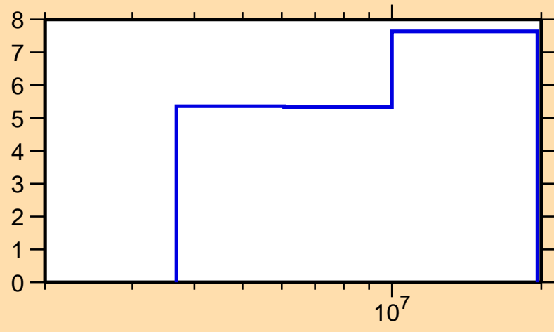
\Delta\sigma/\sigma vs. E for ^{30}\text{P}(n,\text{inel.})
