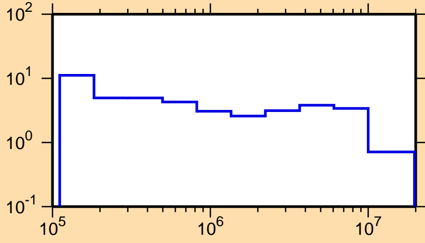
\Delta\sigma/\sigma vs. E for ^{30}\text{P}(n,el.)
