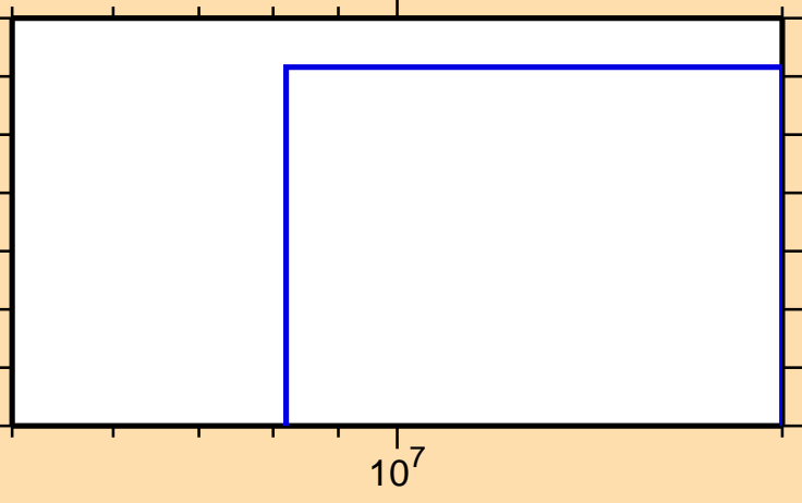
\sigma vs. E for ^{30}\text{P}(n,\text{He}3)
