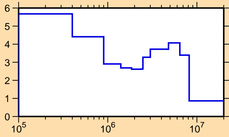
\Delta\sigma/\sigma vs. E for ^{30}\text{P}(n,el.)
