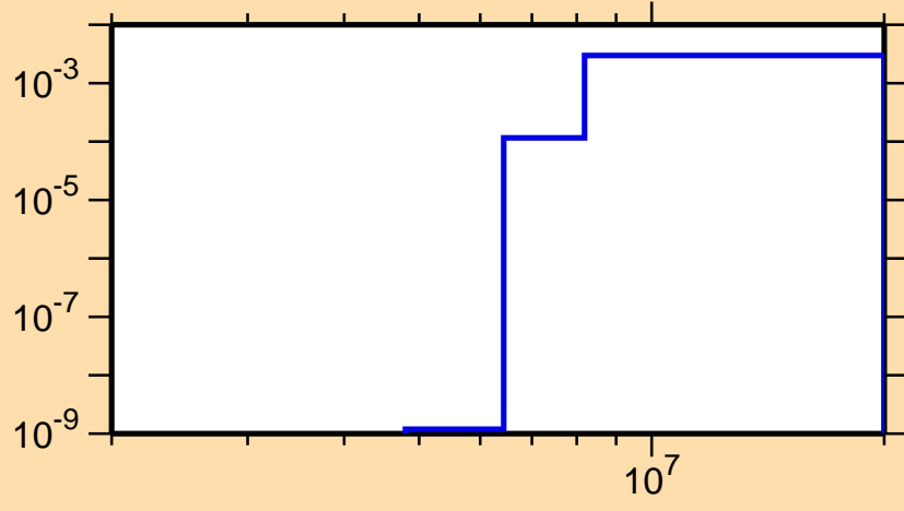
\sigma vs. E for ^{30}\text{P}(n,t)
