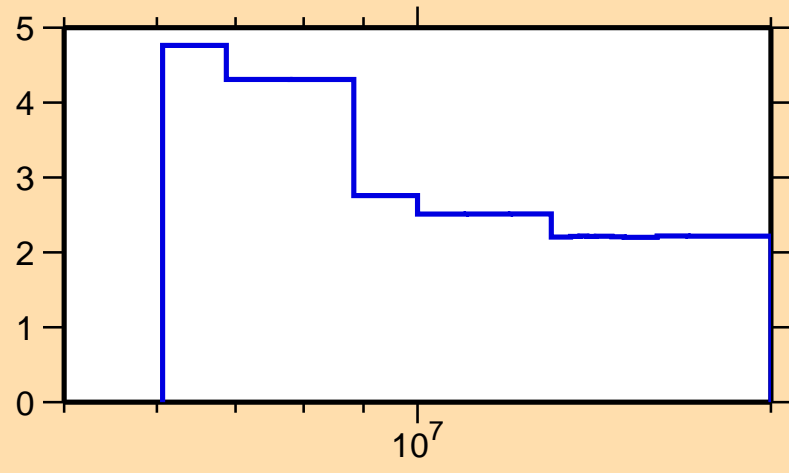
\Delta\sigma/\sigma vs. E for ^{31}\text{P}(n,tot.)
