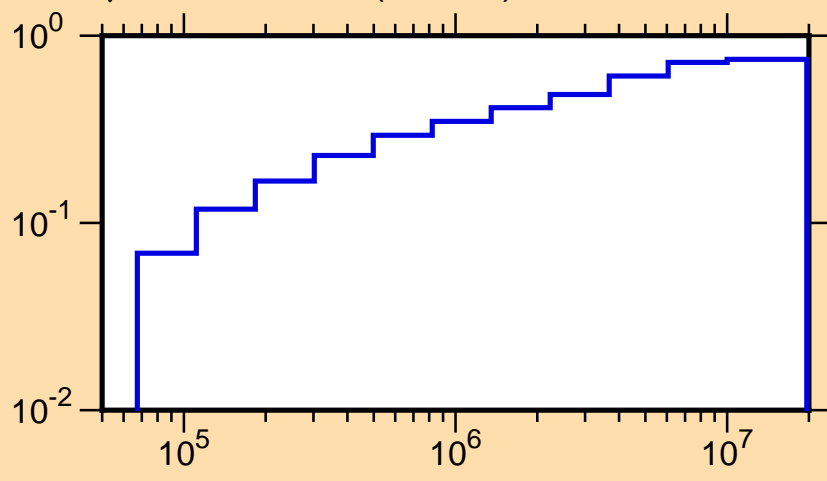
\mu vs. E for ^{31}\text{P} (mt251)
