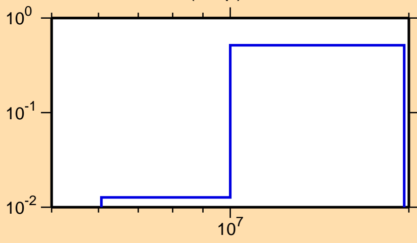
\sigma vs. E for ^{31}\text{P}(n,np)
