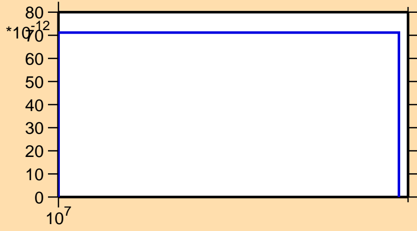
\sigma vs. E for ^{31}\text{P}(n,nt)
