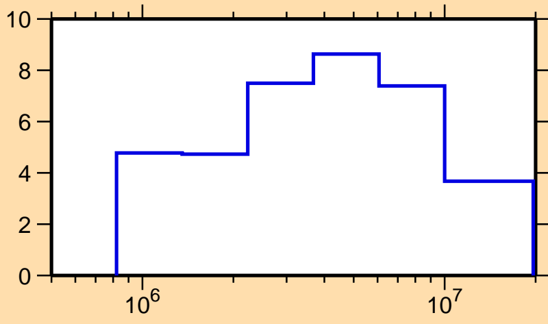
\Delta\sigma/\sigma vs. E for ^{31}\text{P}(n,el.)
