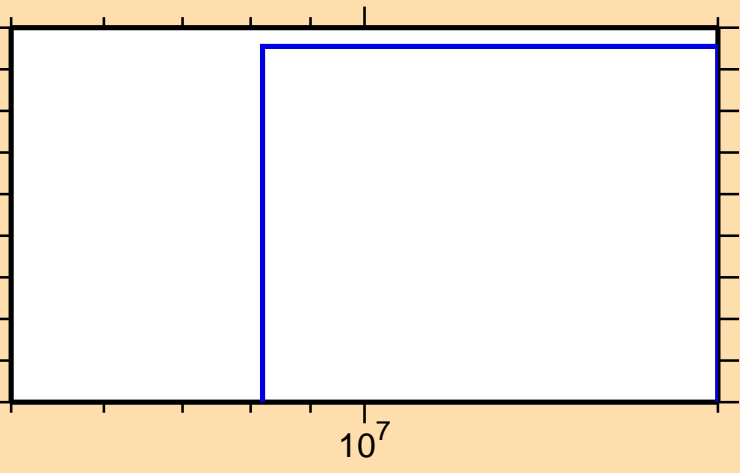
\sigma vs. E for ^{31}\text{P}(n,n\alpha)
