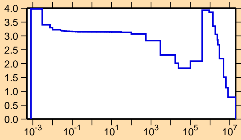
\sigma vs. E for ^{31}\text{P}(n,\text{el.})
