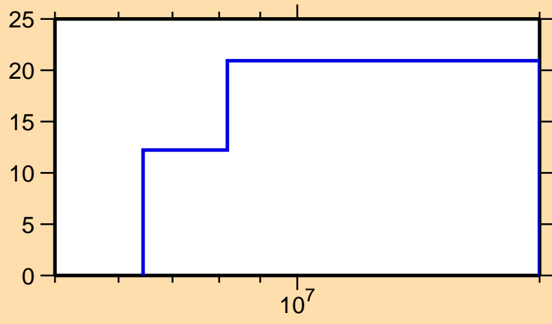
\Delta\sigma/\sigma vs. E for ^{31}\text{P}(n,ncont.)
