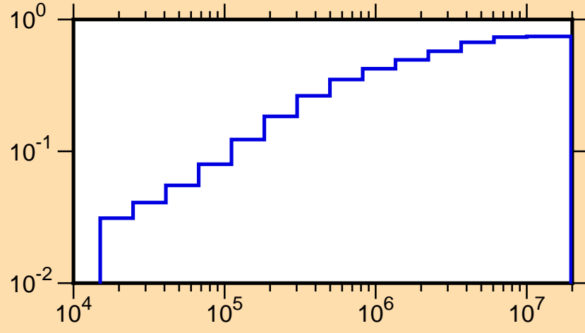
\mu vs. E for ^{32}\text{P}(\text{mt251})
