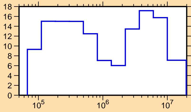
\Delta\sigma/\sigma vs. E for ^{32}\text{P}(n,\text{el.})
