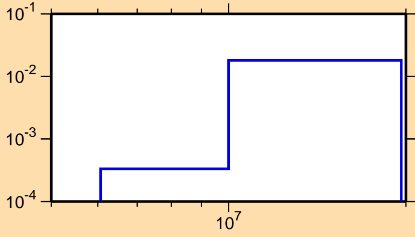
\sigma vs. E for ^{32}\text{P}(n,d)
