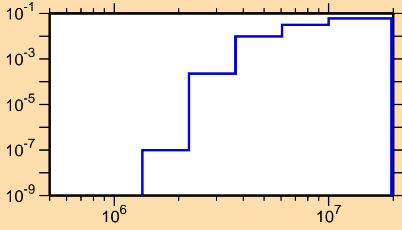
\sigma vs. E for ^{32}\text{P}(n,\alpha)
