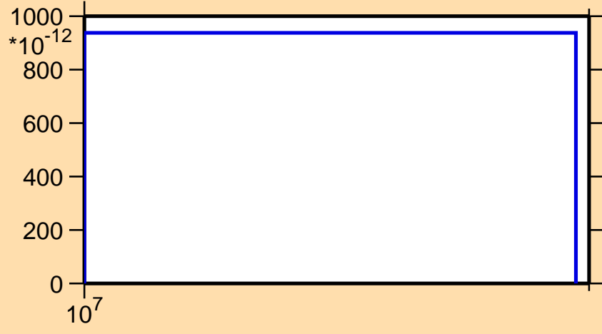
\sigma vs. E for ^{32}\text{P}(n,nt)
