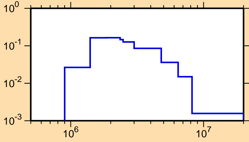
\sigma vs. E for ^{32}\text{P}(n,n_3)
