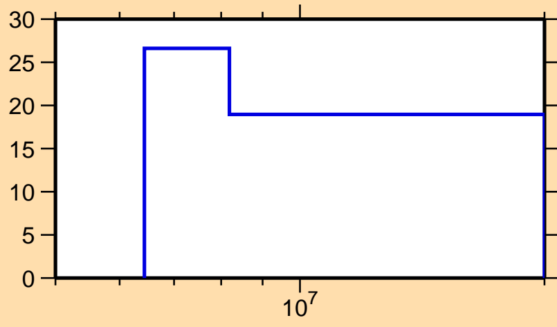
\Delta\sigma/\sigma vs. E for ^{32}\text{P}(n,2n)
