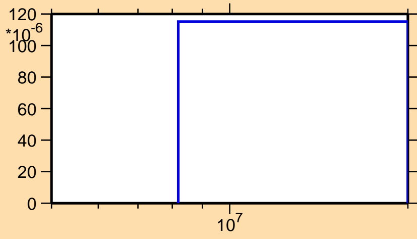
\sigma vs. E for ^{32}\text{P}(n,\text{nd})
