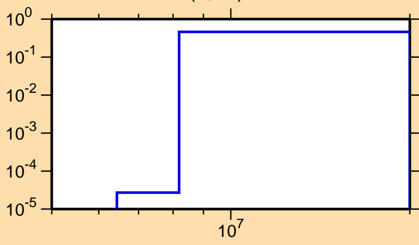
\sigma vs. E for ^{32}\text{P}(n,2n)
