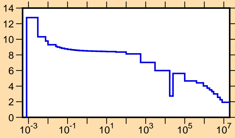
\sigma vs. E for ^{32}\text{P}(n,\text{tot.})
