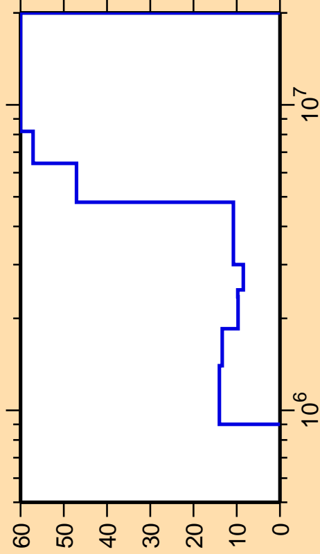
\Delta\sigma/\sigma vs. E for ^{32}\text{P}(n,n_3)
