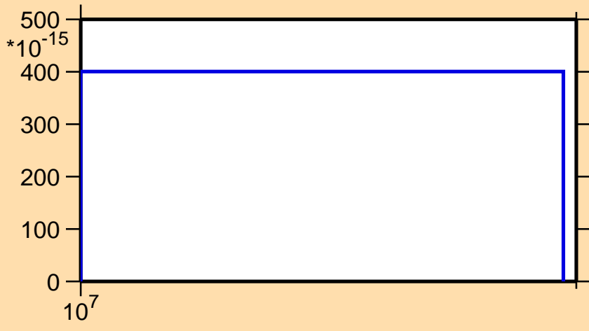
\sigma vs. E for ^{33}\text{P}(n,2np)
