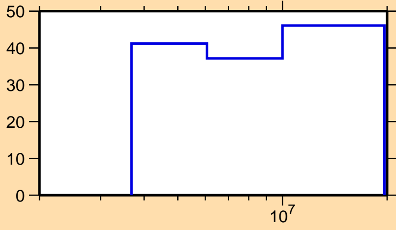
\Delta\sigma/\sigma vs. E for ^{33}\text{P}(n,p)
