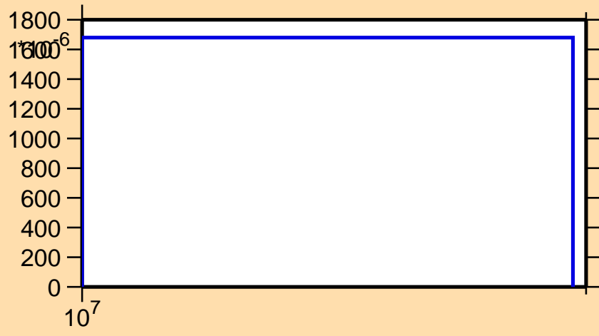
\sigma vs. E for ^{34}\text{P}(n,np)
