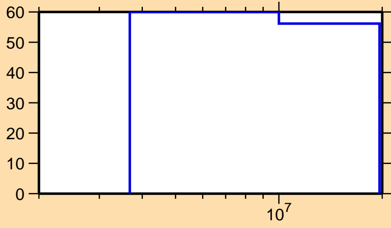
\Delta\sigma/\sigma vs. E for ^{34}\text{P}(n,p)
