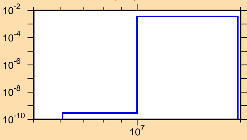
\sigma vs. E for ^{34}\text{P}(n,d)
