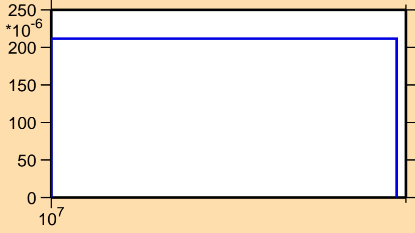
\sigma vs. E for ^{34}\text{P}(n,n\alpha)
