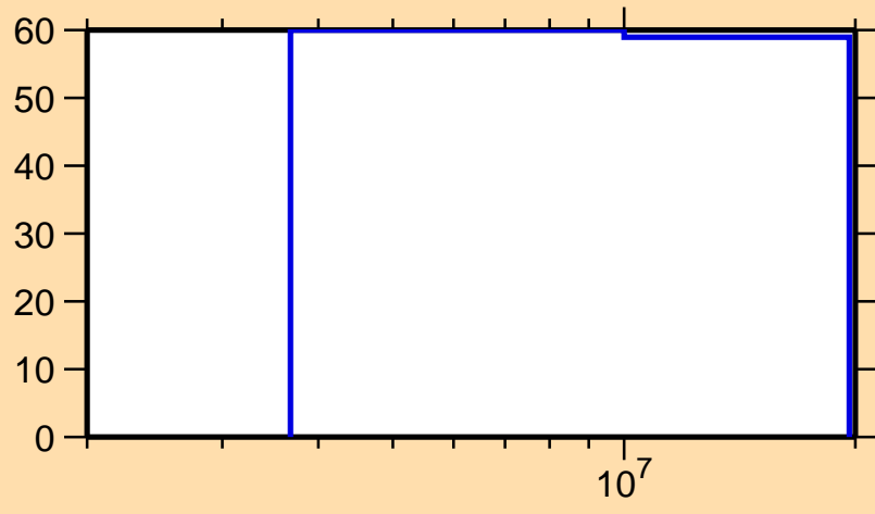
\Delta\sigma/\sigma vs. E for ^{34}\text{P}(n,\gamma)
