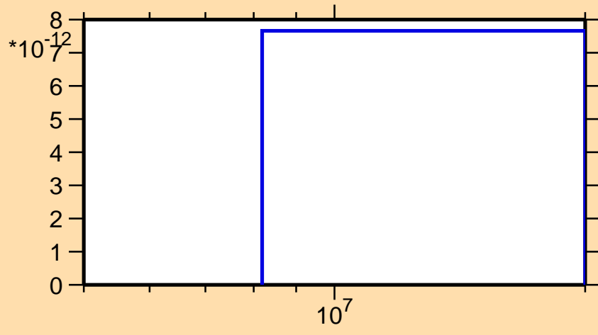
\sigma vs. E for ^{34}\text{P}(n,2n\alpha)
