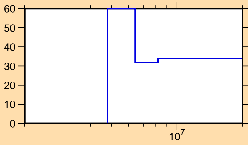
\Delta\sigma/\sigma vs. E for ^{34}\text{P}(n,n\text{cont.})
