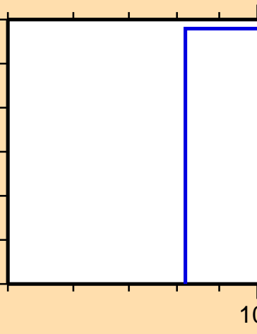
\sigma vs. E for ^{34}\text{P}(n,d)
