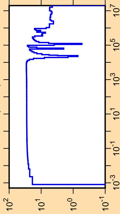
\Delta\sigma/\sigma vs. E for ^{35}\text{P}(n,\text{tot.})
