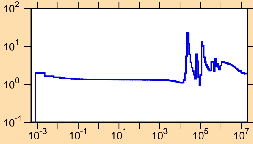
\sigma vs. E for ^{35}\text{P}(n,\text{tot.})
