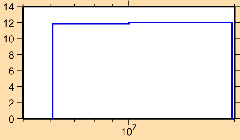
\Delta\sigma/\sigma vs. E for ^{35}\text{P}(n,n\text{onel.})
