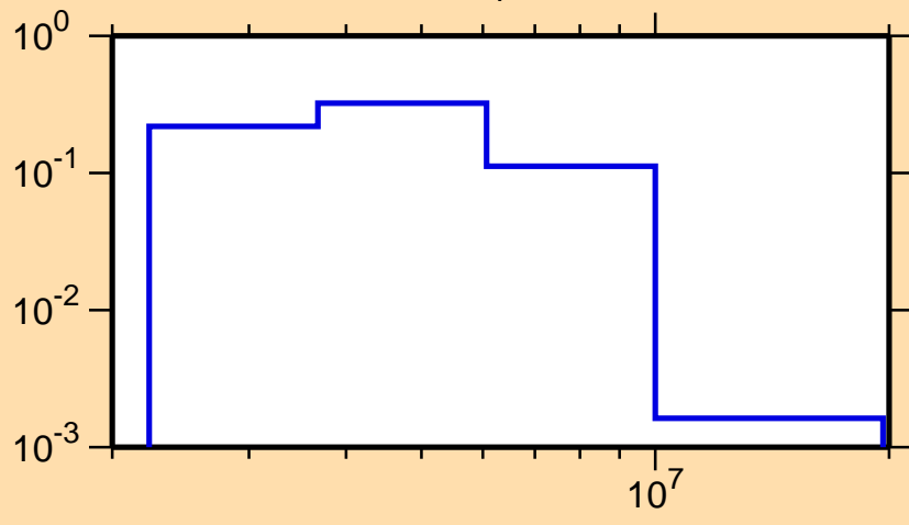
\sigma vs. E for ^{35}\text{P}(n,n_1)
