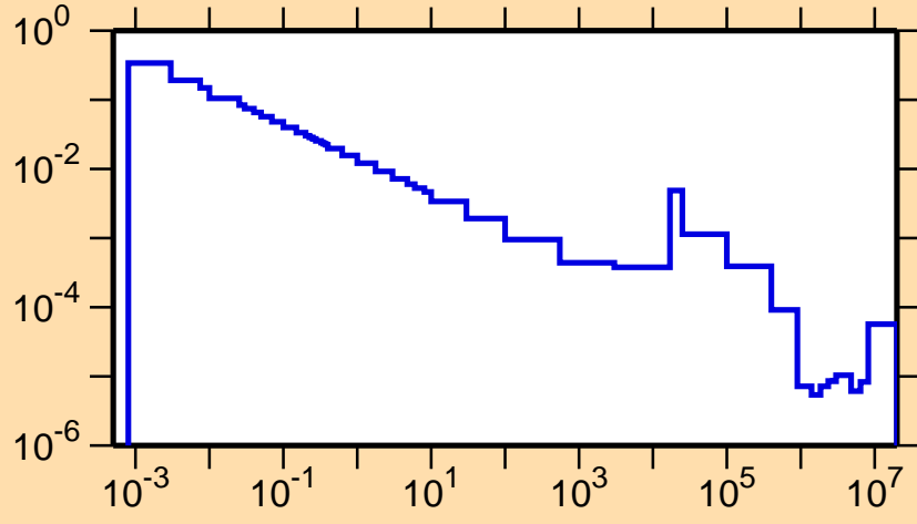
\sigma vs. E for ^{35}\text{P}(n,\gamma)
