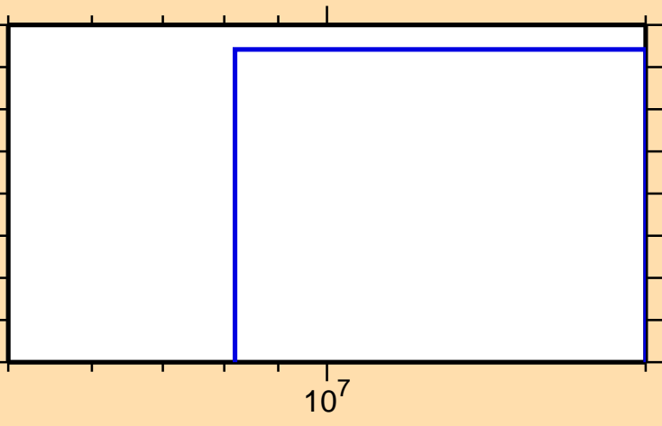
\sigma vs. E for ^{35}\text{P}(n,np)
