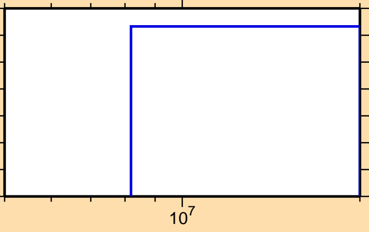
\sigma vs. E for ^{37}\text{P}(n,\alpha)
