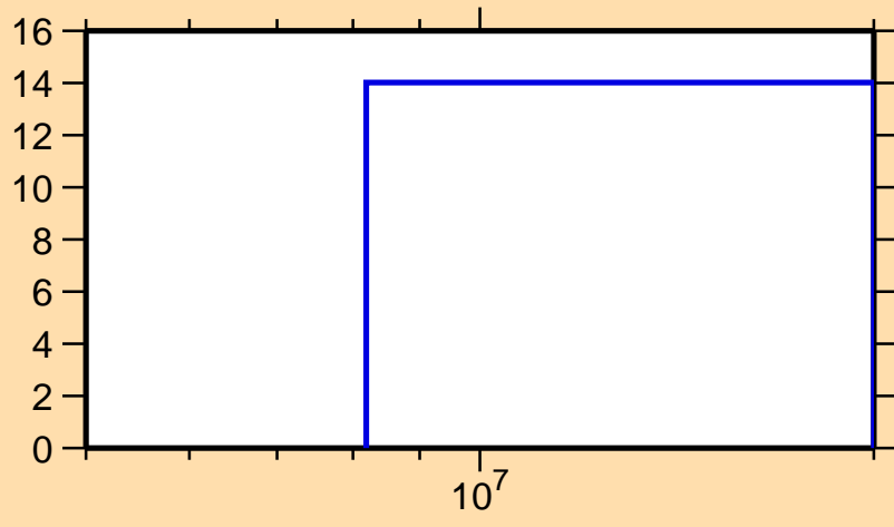
\Delta\sigma/\sigma vs. E for ^{37}\text{P}(n,n\text{onel.})
