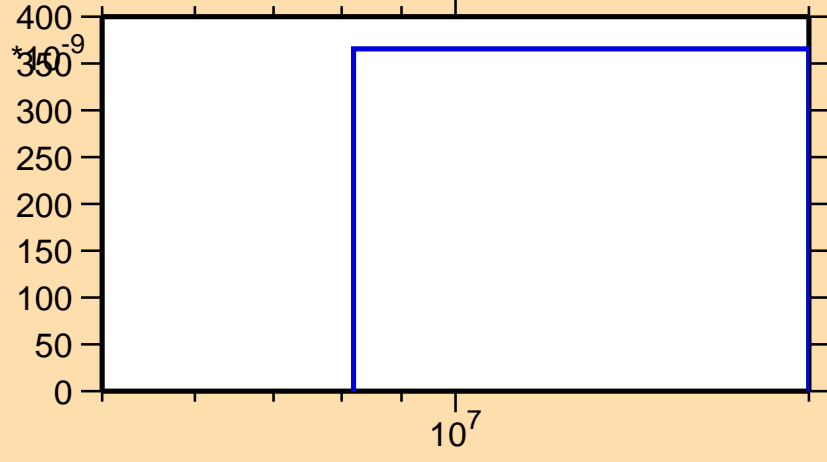
\sigma vs. E for ^{37}\text{P}(n,nt)
