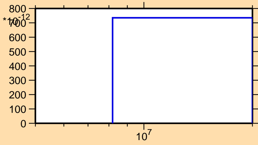
\sigma vs. E for ^{37}\text{P}(n,\text{nd})
