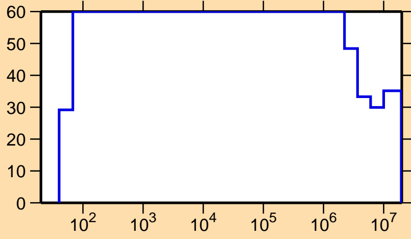
\Delta\sigma/\sigma vs. E for ^{225}\text{Pa}(n,p)
