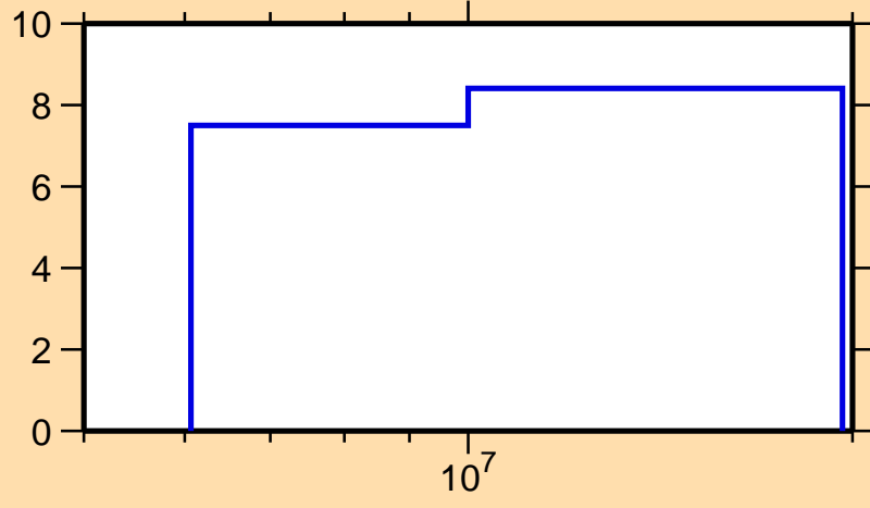
\Delta\sigma/\sigma vs. E for ^{225}\text{Pa}(n,\text{nonel.})
