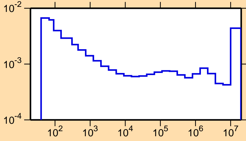
\sigma vs. E for ^{225}\text{Pa}(n,\alpha)
