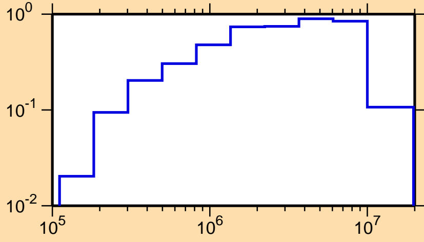
\sigma vs. E for ^{225}\text{Pa}(n,\text{inel.})
