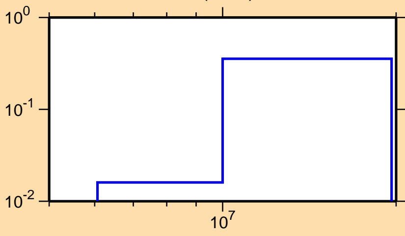
\sigma vs. E for ^{225}\text{Pa}(n,2n)
