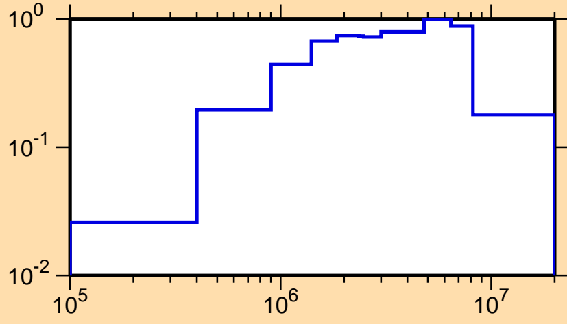
\sigma vs. E for ^{225}\text{Pa}(n,n\text{cont.})
