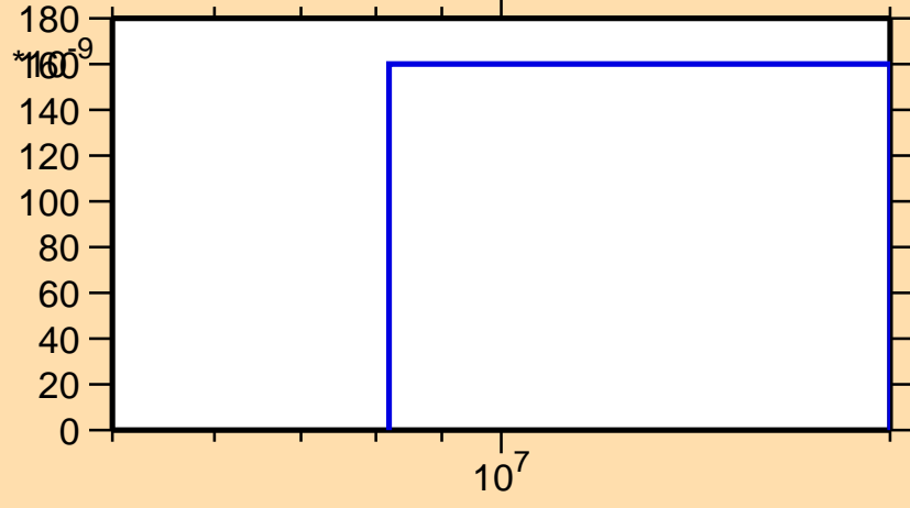
\sigma vs. E for ^{225}\text{Pa}(n,nd)
