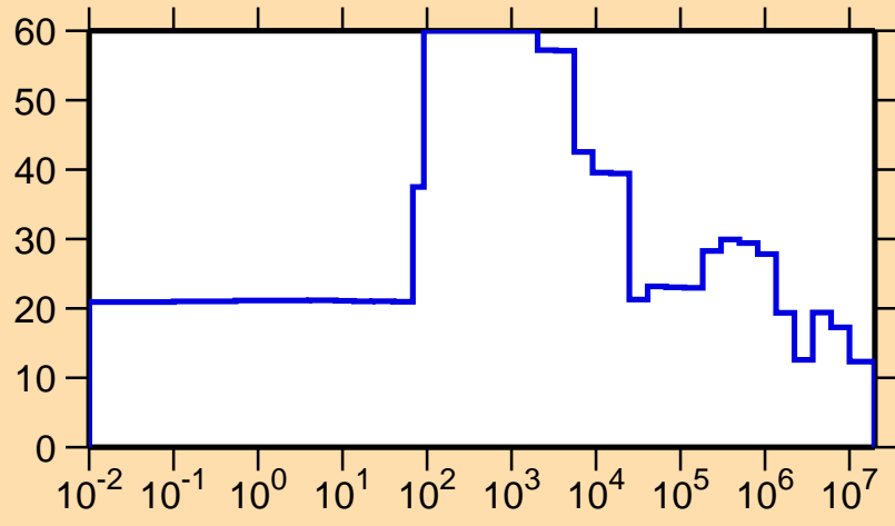
\Delta\sigma/\sigma vs. E for ^{226}\text{Pa}(n,el.)
