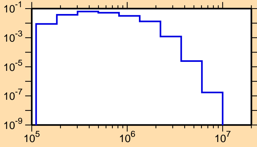
\sigma vs. E for ^{226}\text{Pa}(n,n_1)
