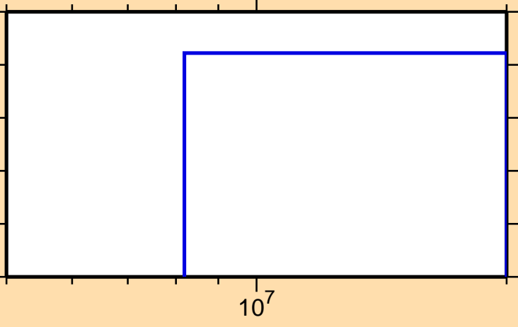
\sigma vs. E for ^{226}\text{Pa}(n,2np)
