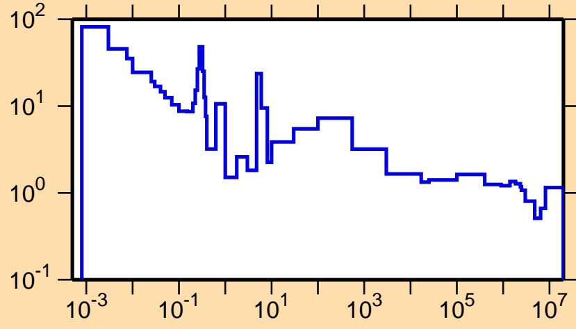
\sigma vs. E for ^{226}\text{Pa}(n,f)
