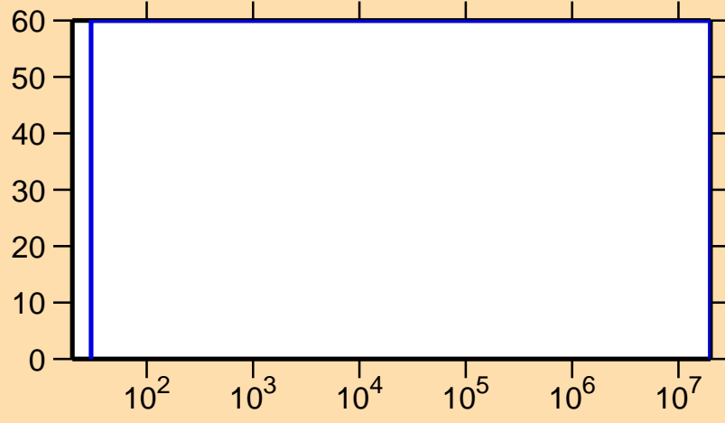
\Delta\sigma/\sigma vs. E for ^{226}\text{Pa}(n,\gamma)
