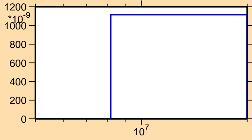
\sigma vs. E for ^{226}\text{Pa}(n,nd)
