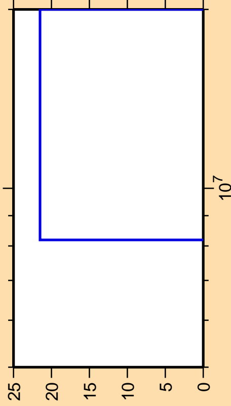
\Delta\sigma/\sigma vs. E for ^{226}\text{Pa}(n,nd)
