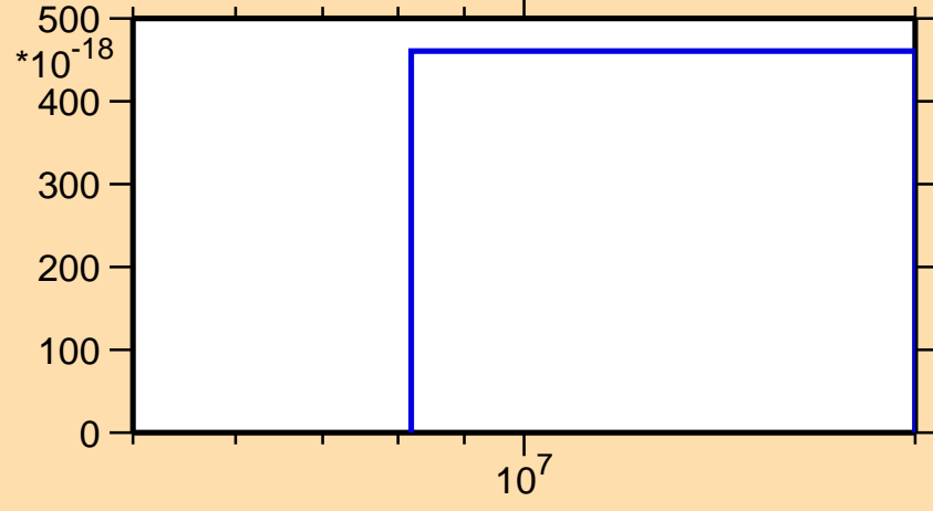
\sigma vs. E for ^{226}\text{Pa}(\text{mt } 42)
