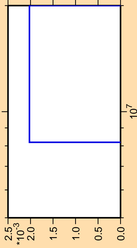
\Delta\sigma/\sigma vs. E for ^{226}\text{Pa}(\text{mt } 42)
