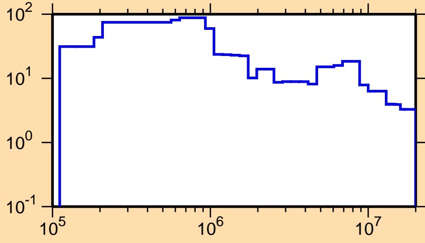
\Delta\sigma/\sigma vs. E for ^{227}\text{Pa}(n,\text{el.})
