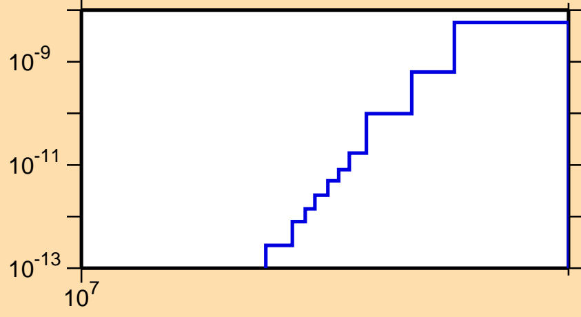
\sigma vs. E for ^{227}\text{Pa}(n,\text{He3})
