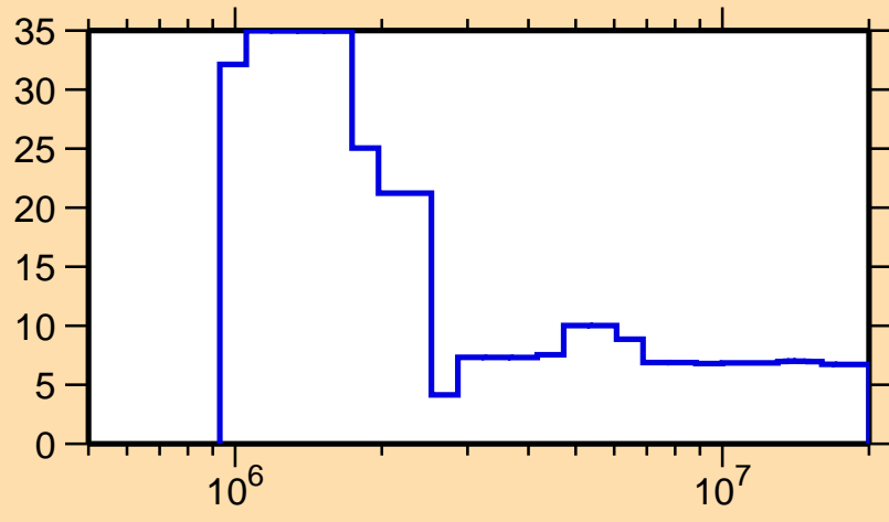
\Delta\sigma/\sigma vs. E for ^{227}\text{Pa}(n,\text{nonel.})
