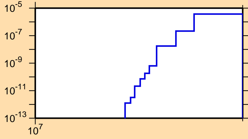
\sigma vs. E for ^{227}\text{Pa}(n,2np)
