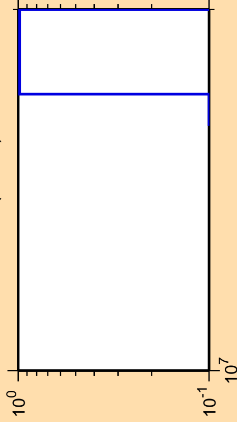
\Delta\sigma/\sigma vs. E for ^{227}\text{Pa} (mt 42)
