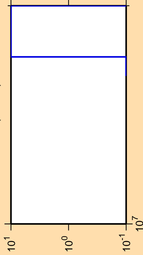
\Delta\sigma/\sigma vs. E for ^{227}\text{Pa} (mt 11)
