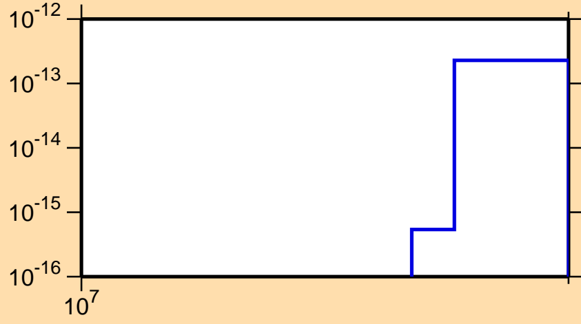
\sigma vs. E for ^{227}\text{Pa} (mt 34)
