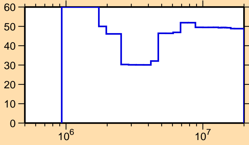
\Delta\sigma/\sigma vs. E for ^{227}\text{Pa}(n,\text{inel.})
