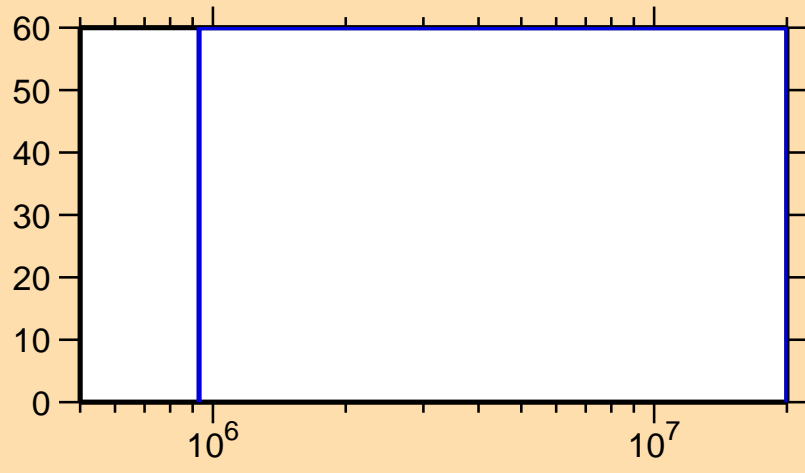
\Delta\sigma/\sigma vs. E for ^{227}\text{Pa}(n,\gamma)
