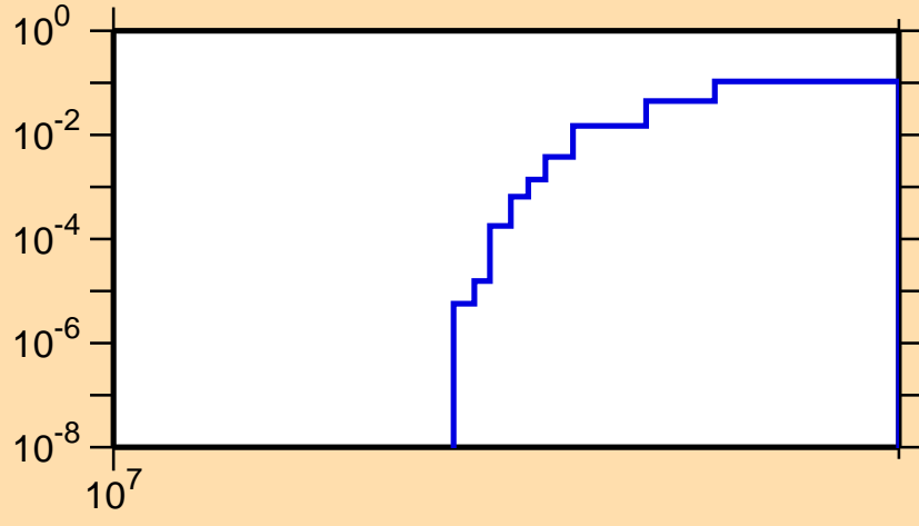
\sigma vs. E for ^{227}\text{Pa}(n,3n\alpha)
