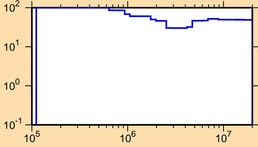
\Delta\sigma/\sigma vs. E for ^{227}\text{Pa}(n,\text{inel.})
