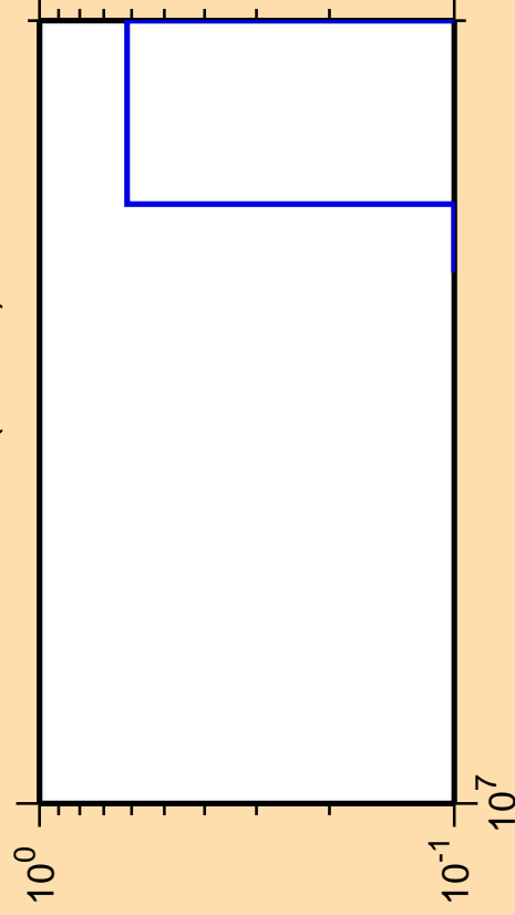
\Delta\sigma/\sigma vs. E for ^{227}\text{Pa} (mt 34)
