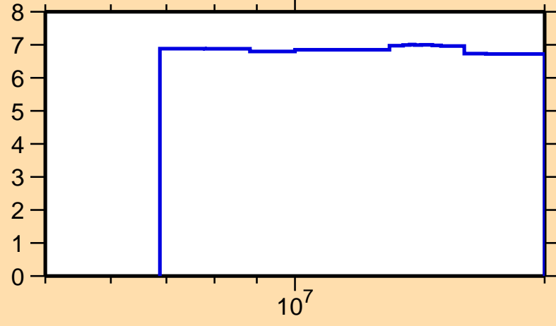
\Delta\sigma/\sigma vs. E for ^{227}\text{Pa}(n,\text{nonel.})
