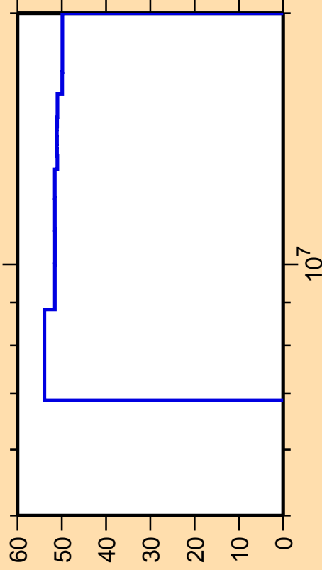
\Delta\sigma/\sigma vs. E for ^{227}\text{Pa}(n,n\text{cont.})
