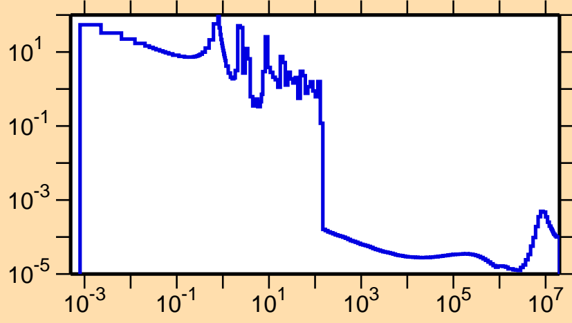
\sigma vs. E for ^{227}\text{Pa}(n,\gamma)
