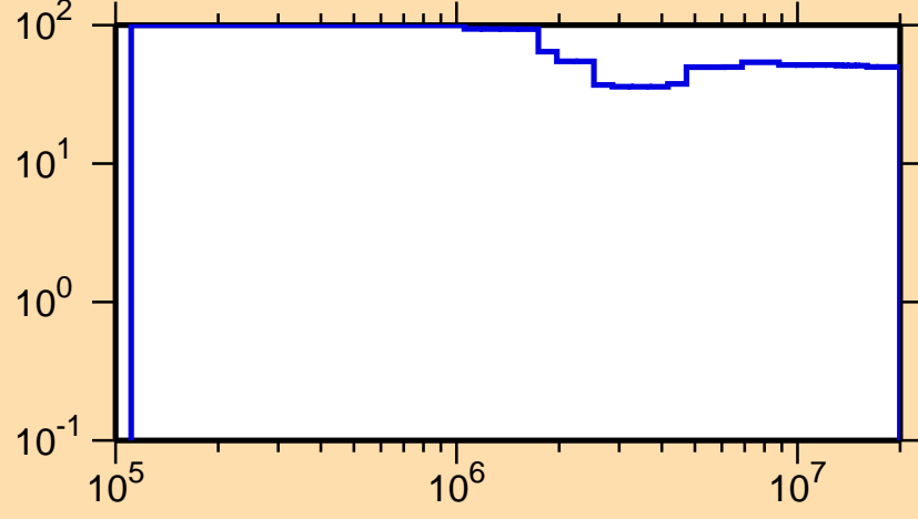
\Delta\sigma/\sigma vs. E for ^{227}\text{Pa}(n,n\text{cont.})
