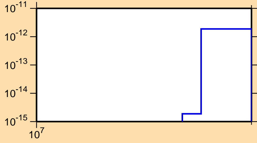
\sigma vs. E for ^{227}\text{Pa} (mt 11)
