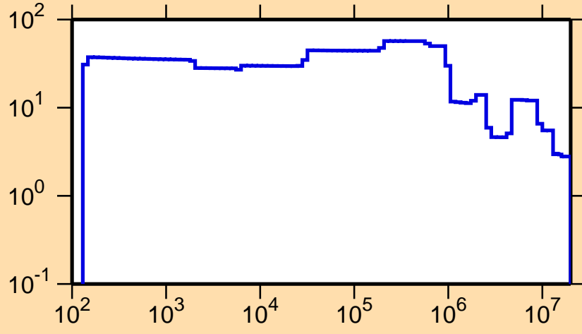
\Delta\sigma/\sigma vs. E for ^{227}\text{Pa}(n,\text{tot.})
