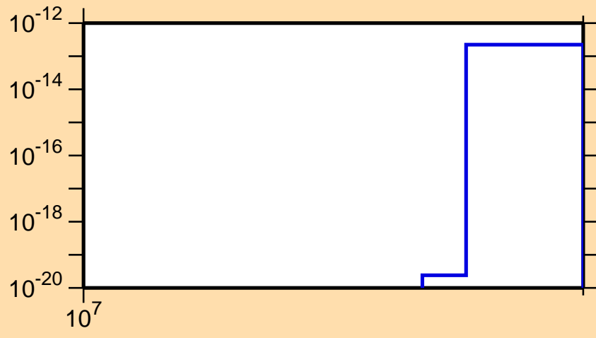
\sigma vs. E for ^{227}\text{Pa} (mt 42)
