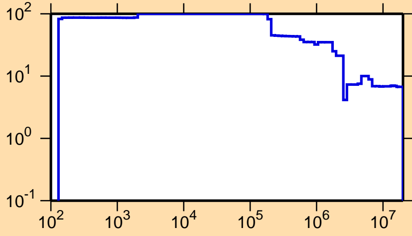
\Delta\sigma/\sigma vs. E for ^{227}\text{Pa}(n,\text{nonel.})
