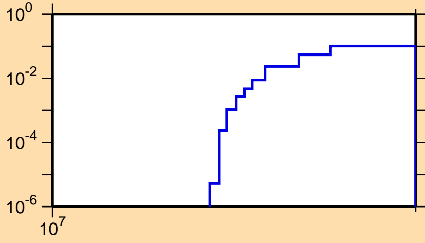
\sigma vs. E for ^{227}\text{Pa}(n,3n)
