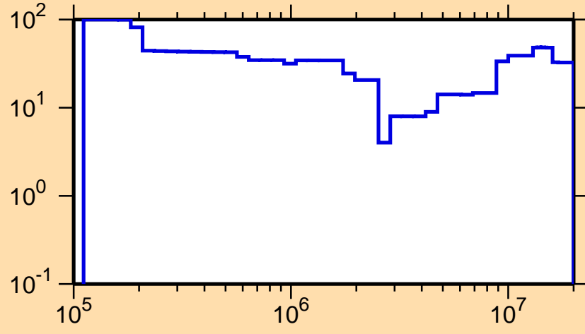
\Delta\sigma/\sigma vs. E for ^{227}\text{Pa}(n,f)
