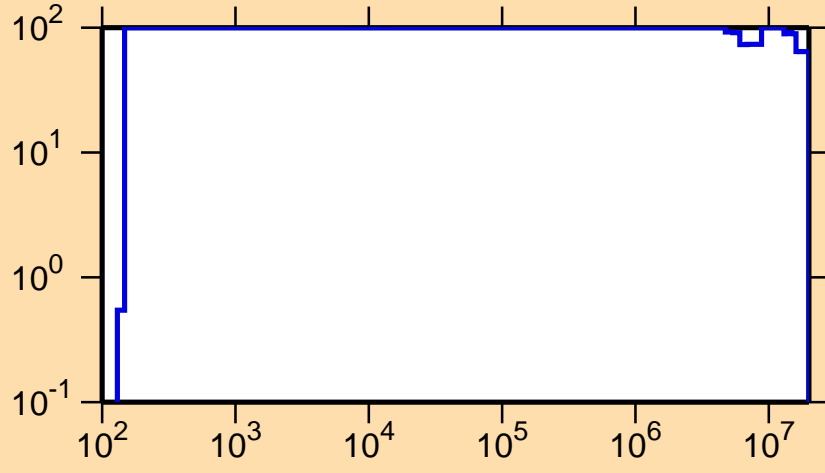
\Delta\sigma/\sigma vs. E for ^{227}\text{Pa}(n,\gamma)
