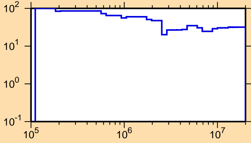
\Delta\sigma/\sigma vs. E for ^{227}\text{Pa}(n,n_1)
