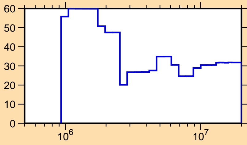
\Delta\sigma/\sigma vs. E for ^{227}\text{Pa}(n,n_1)
