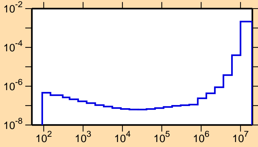
\sigma vs. E for ^{227}\text{Pa}(n,\alpha)
