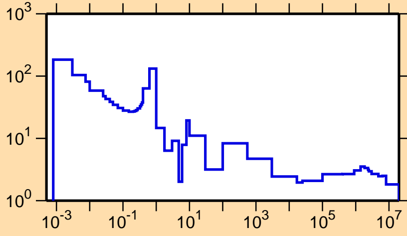
\sigma vs. E for ^{227}\text{Pa}(n,f)
