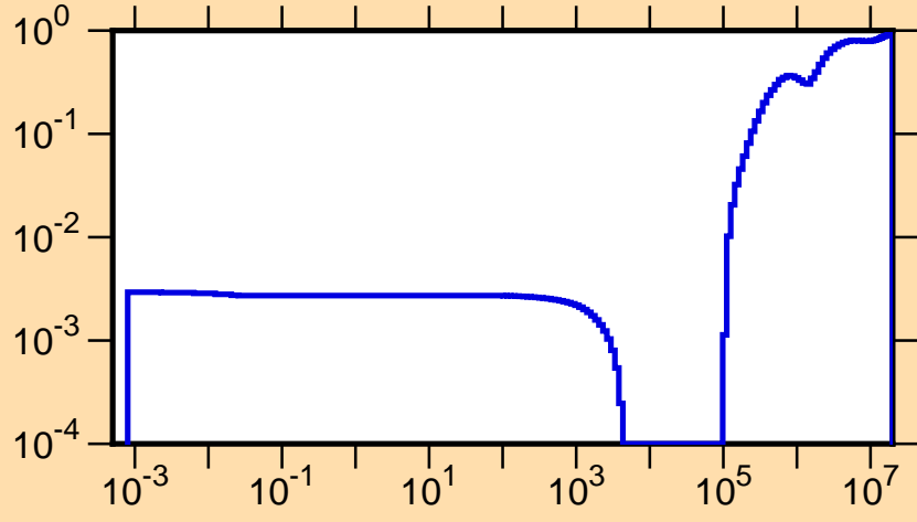
\mu vs. E for ^{228}\text{Pa}(\text{mt251})
