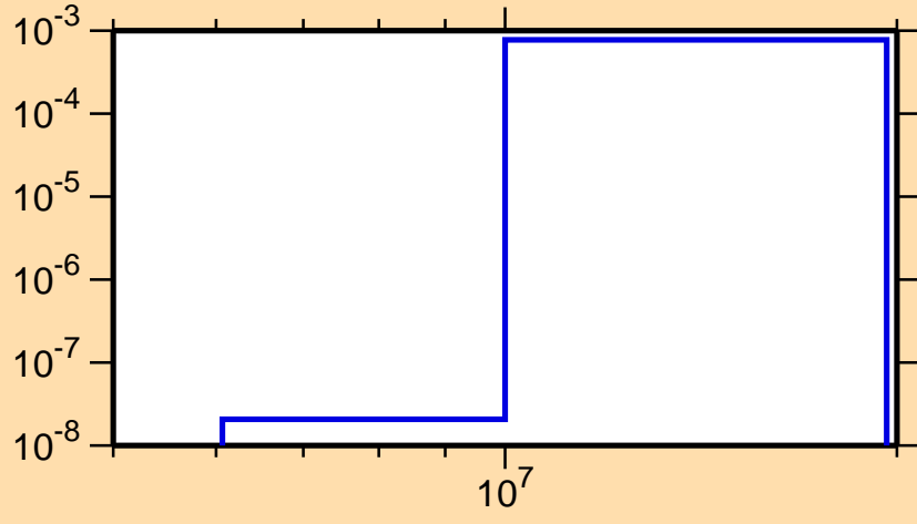
\sigma vs. E for ^{228}\text{Pa}(n,d)
