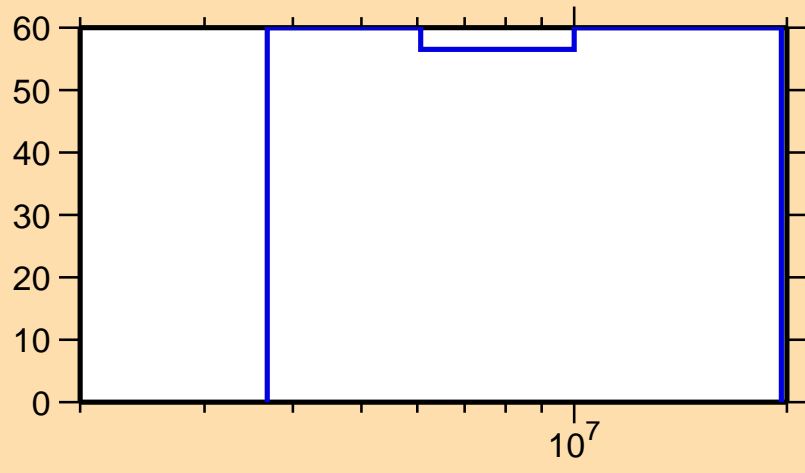
\Delta\sigma/\sigma vs. E for ^{228}\text{Pa}(n,2n)
