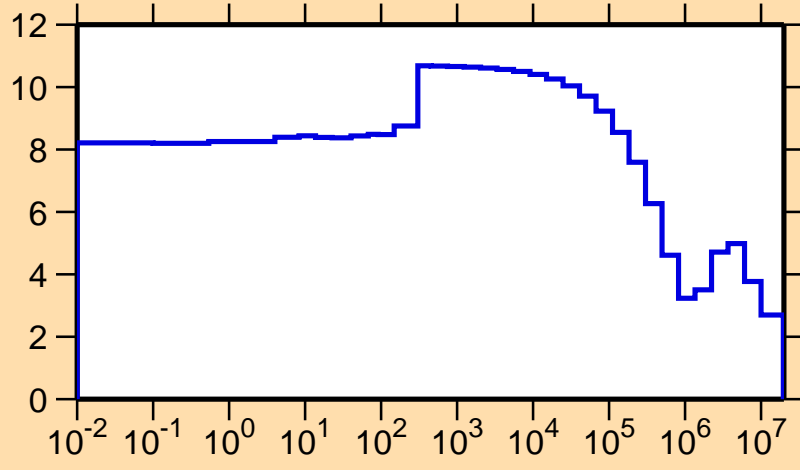
\sigma vs. E for ^{228}\text{Pa}(n,\text{el.})
