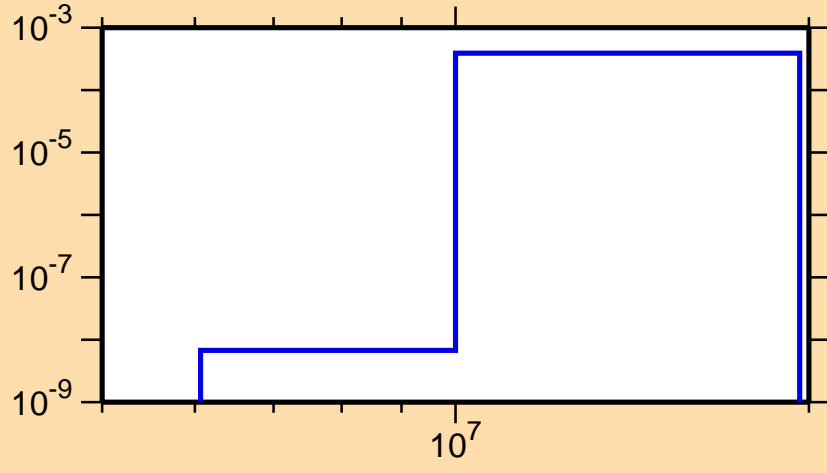
\sigma vs. E for ^{228}\text{Pa}(n,np)
