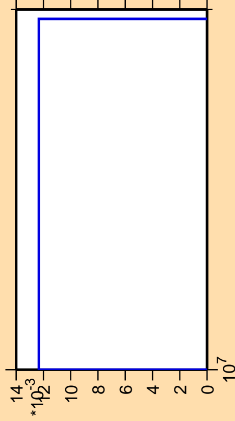
\Delta\sigma/\sigma vs. E for ^{228}\text{Pa} (mt 11)
