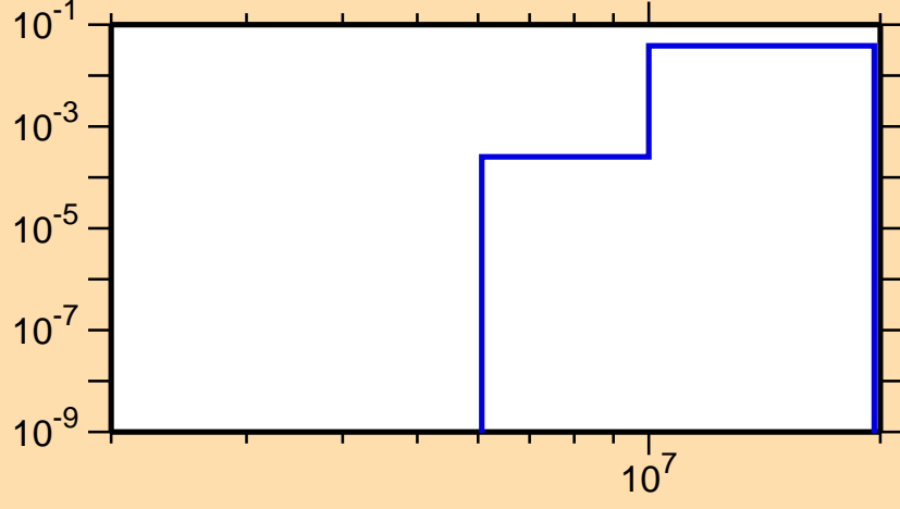
\sigma vs. E for ^{228}\text{Pa}(n,2n\alpha)
