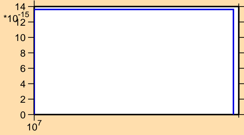
\sigma vs. E for ^{228}\text{Pa} (mt 11)
