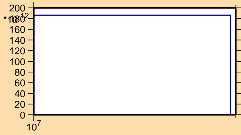
\sigma vs. E for ^{228}\text{Pa}(n,\text{He3})
