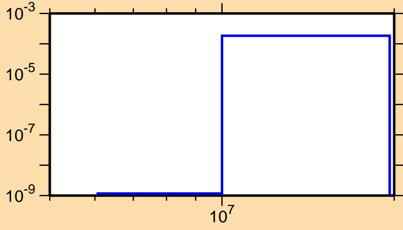
\sigma vs. E for ^{228}\text{Pa}(n,t)
