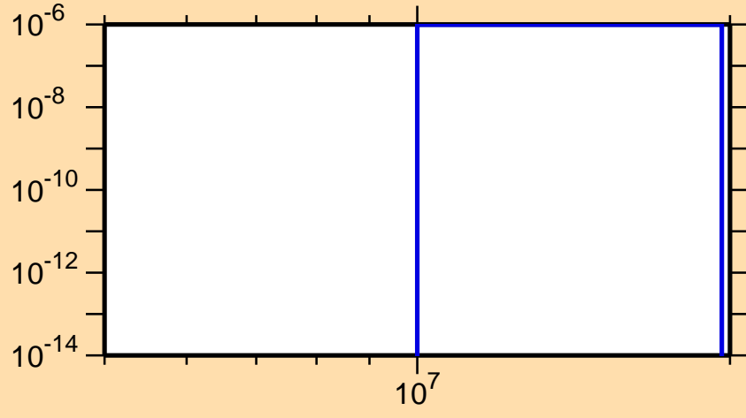
\sigma vs. E for ^{228}\text{Pa}(n,nd)
