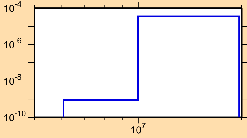
\sigma vs. E for ^{228}\text{Pa}(\text{mt117})
