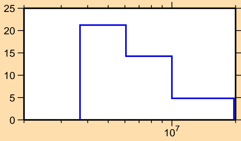
\Delta\sigma/\sigma vs. E for ^{228}\text{Pa}(n,\text{tot.})
