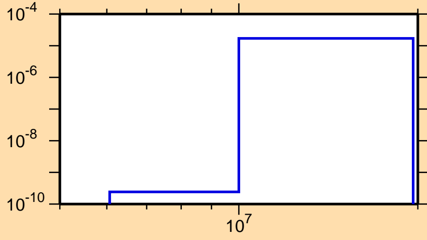
\sigma vs. E for ^{228}\text{Pa} (mt 45)
