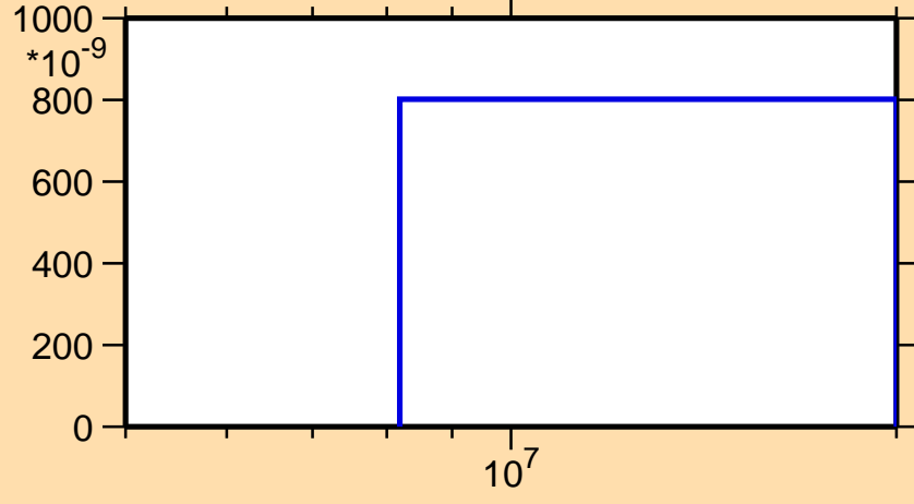
\sigma vs. E for ^{228}\text{Pa}(n,nd)
