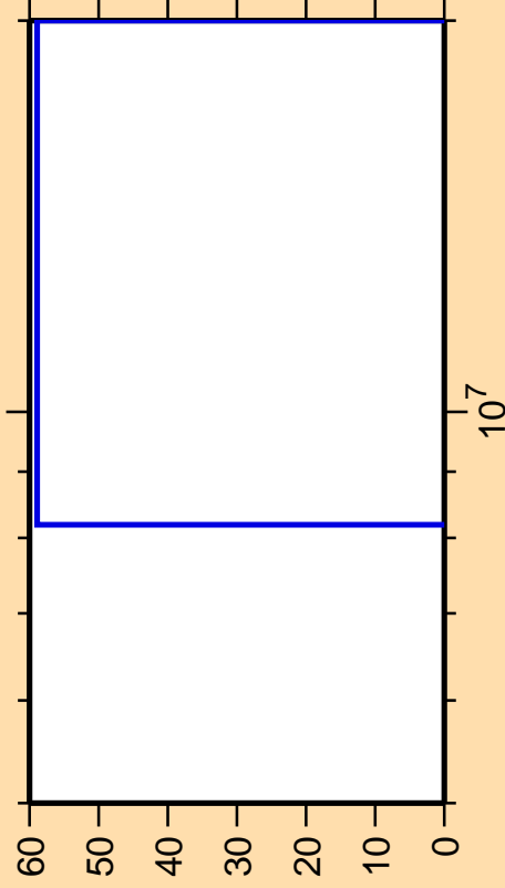
\Delta\sigma/\sigma vs. E for ^{228}\text{Pa}(n,nd)
