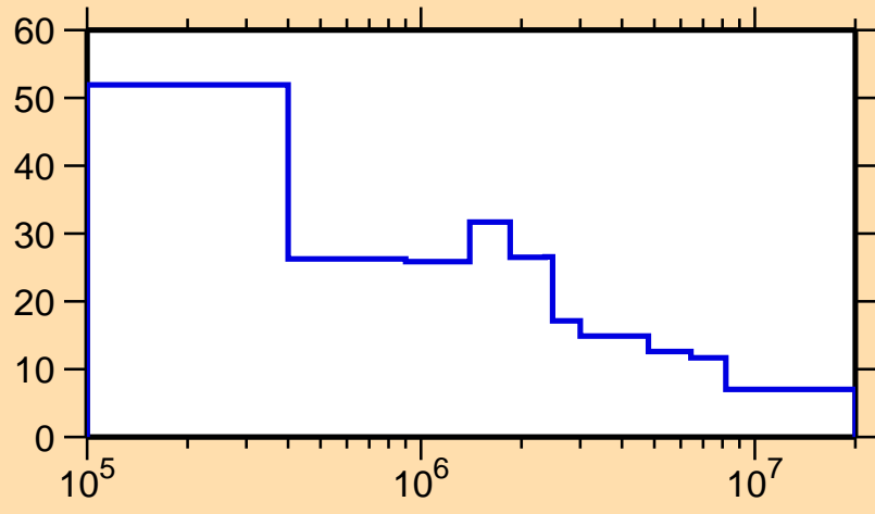
\Delta\sigma/\sigma vs. E for ^{228}\text{Pa}(n,\text{nonel.})
