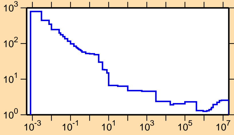
\sigma vs. E for ^{228}\text{Pa}(n,f)
