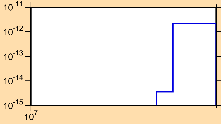
\sigma vs. E for ^{229}\text{Pa} (mt 11)
