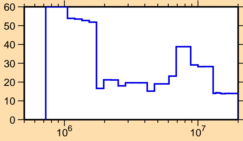
\Delta\sigma/\sigma vs. E for ^{229}\text{Pa}(n,el.)
