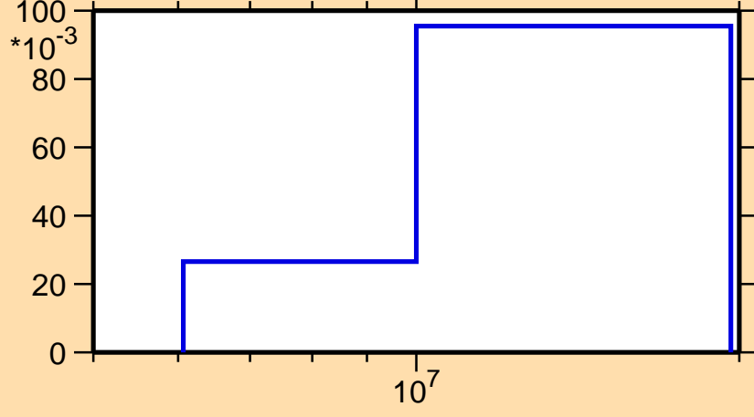
\sigma vs. E for ^{229}\text{Pa}(n,2n)
