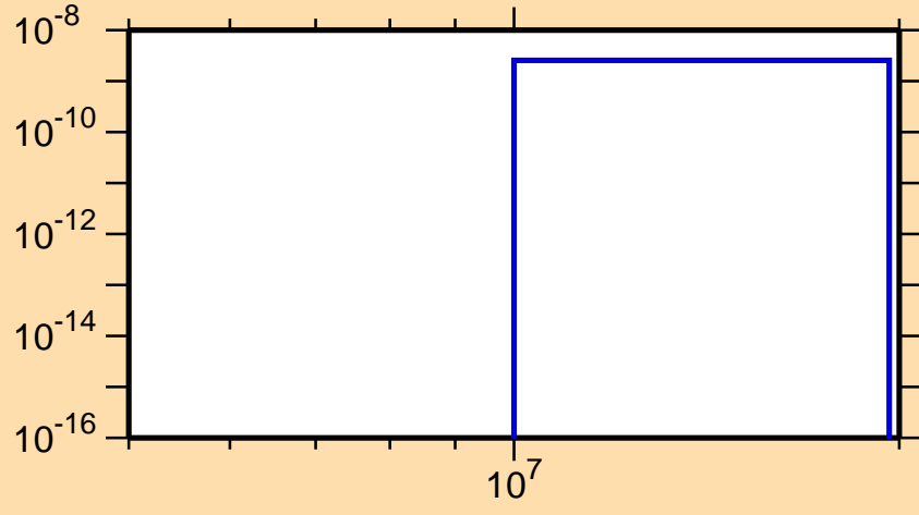
\sigma vs. E for ^{229}\text{Pa}(\text{mt117})
