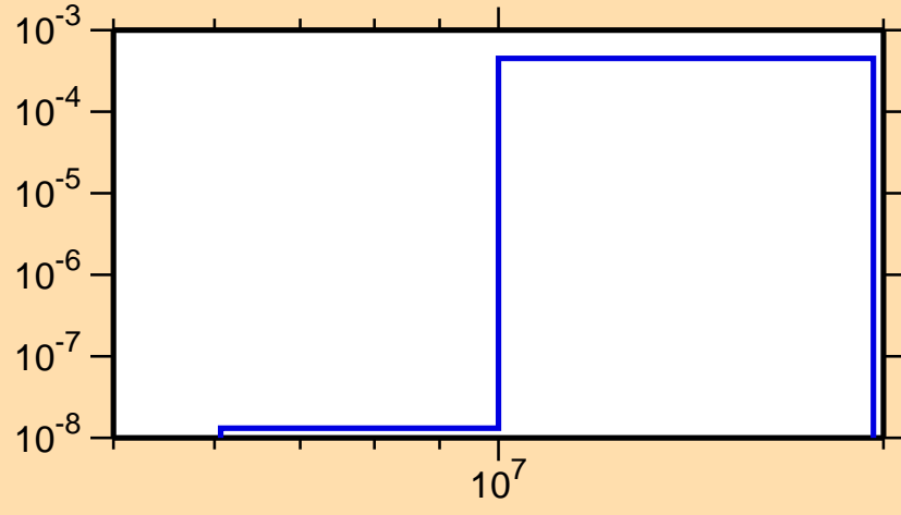
\sigma vs. E for ^{229}\text{Pa}(n,d)
