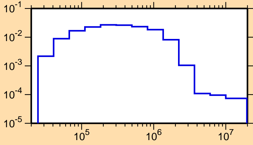
\sigma vs. E for ^{229}\text{Pa}(n,n_3)
