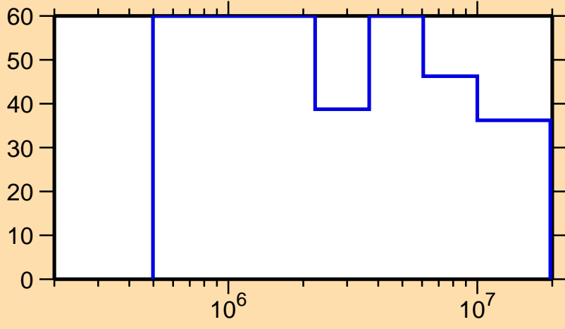
\Delta\sigma/\sigma vs. E for ^{229}\text{Pa}(n,n_1)
