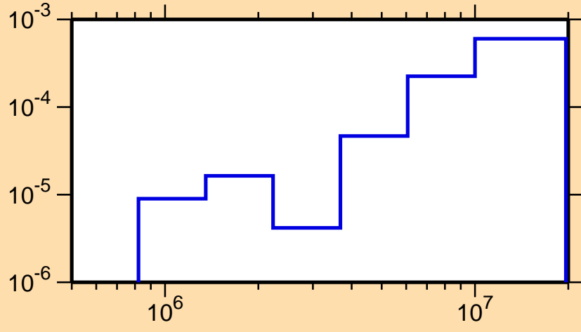
\sigma vs. E for ^{229}\text{Pa}(n,n\alpha)
