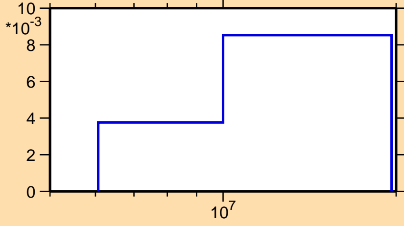
\sigma vs. E for ^{229}\text{Pa}(n,2n\alpha)
