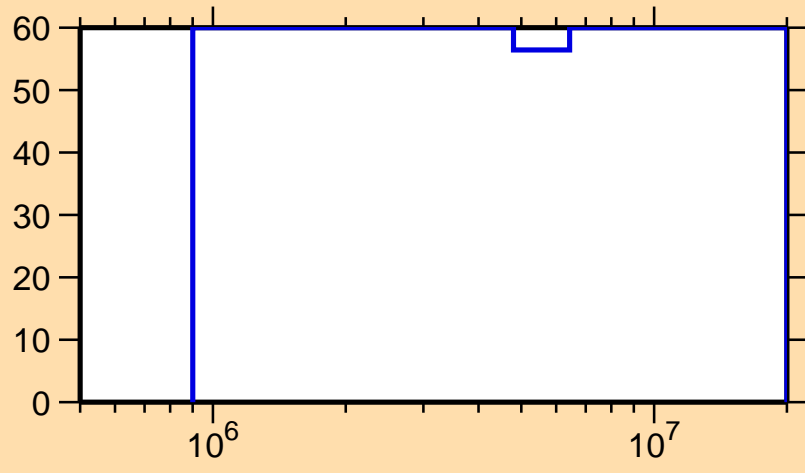
\Delta\sigma/\sigma vs. E for ^{230}\text{Pa}(n,n_1)
