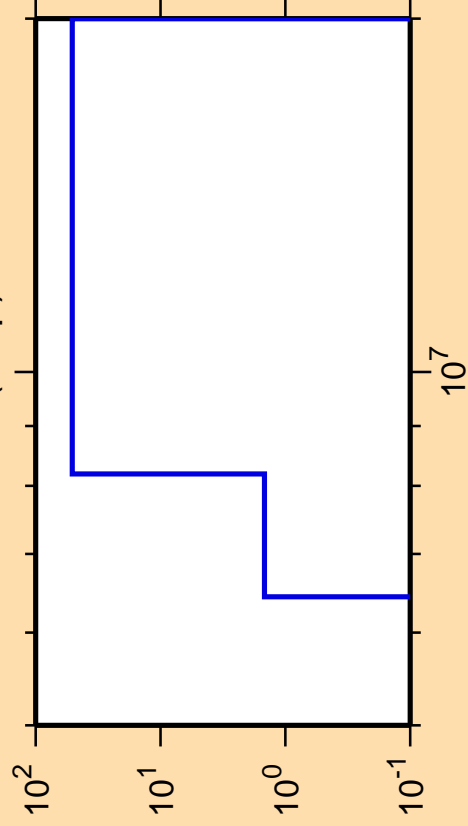
\Delta\sigma/\sigma vs. E for ^{230}\text{Pa}(n,np)
