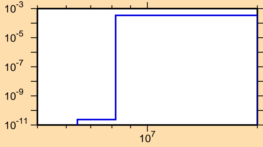
\sigma vs. E for ^{230}\text{Pa}(n,d)
