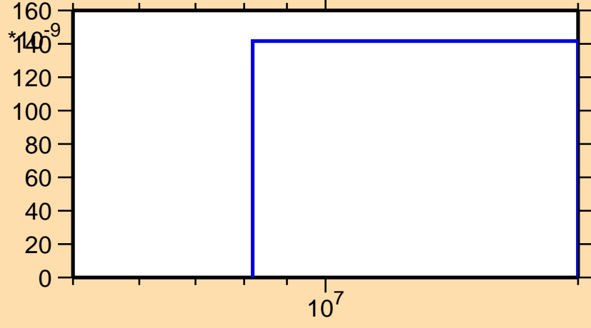
\sigma vs. E for ^{230}\text{Pa}(n,2np)
