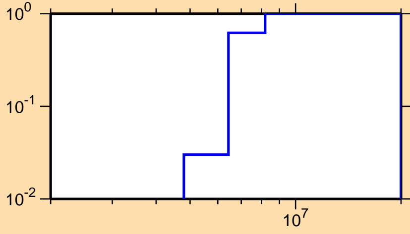
\sigma vs. E for ^{230}\text{Pa}(n,2n)
