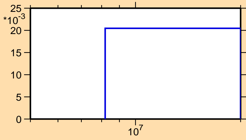
\sigma vs. E for ^{230}\text{Pa}(n,3n)
