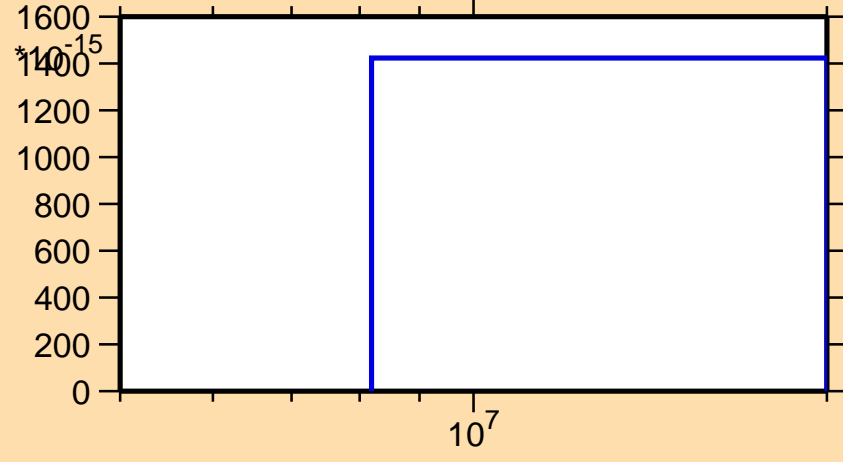
\sigma vs. E for ^{230}\text{Pa} (mt 45)
