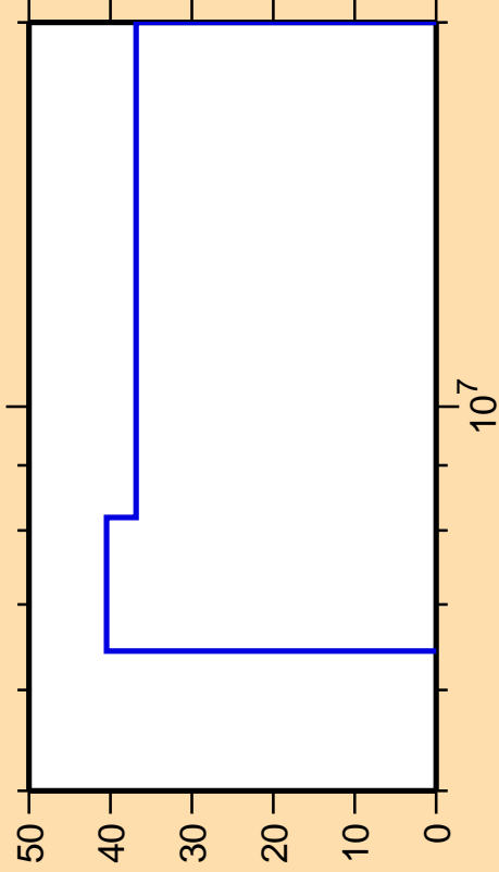
\Delta\sigma/\sigma vs. E for ^{230}\text{Pa}(n,d)
