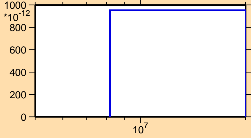
\sigma vs. E for ^{230}\text{Pa}(n,p\alpha)
