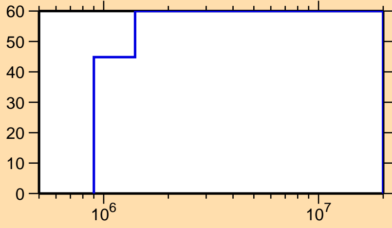
\Delta\sigma/\sigma vs. E for ^{230}\text{Pa}(n,p)
