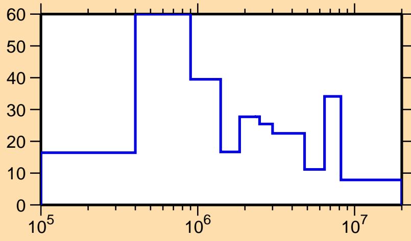
\Delta\sigma/\sigma vs. E for ^{230}\text{Pa}(n,\text{el.})
