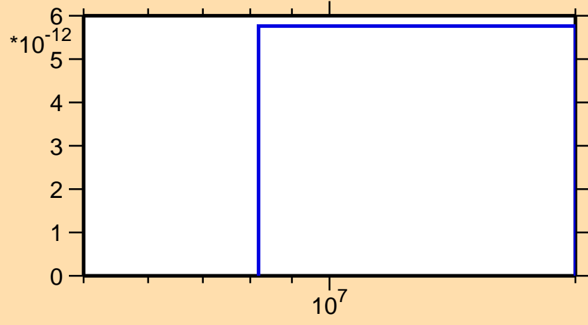
\sigma vs. E for ^{230}\text{Pa}(\text{mt117})
