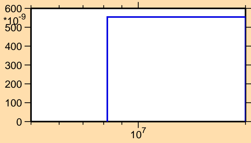
\sigma vs. E for ^{230}\text{Pa}(n,\text{nd})
