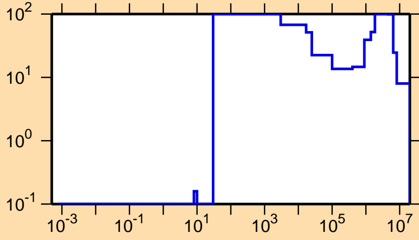
\Delta\sigma/\sigma vs. E for ^{230}\text{Pa}(n,f)
