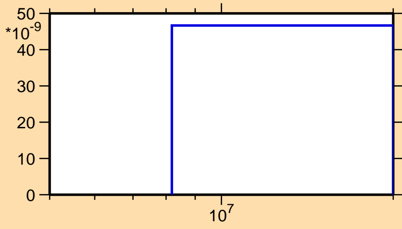
\sigma vs. E for ^{230}\text{Pa}(n,nt)
