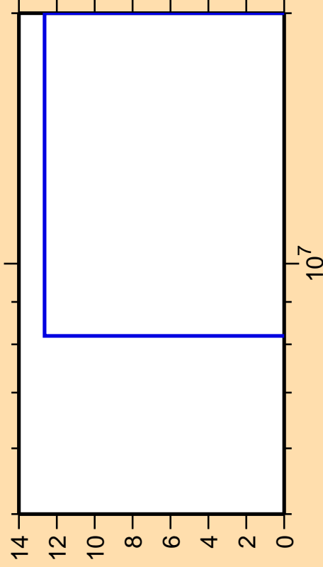
\Delta\sigma/\sigma vs. E for ^{230}\text{Pa} (mt 45)
