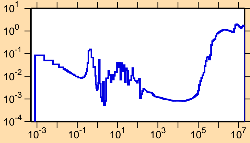
\sigma vs. E for ^{231}\text{Pa}(n,f)
