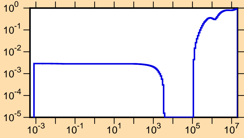
\mu vs. E for ^{232}\text{Pa}(\text{mt251})
