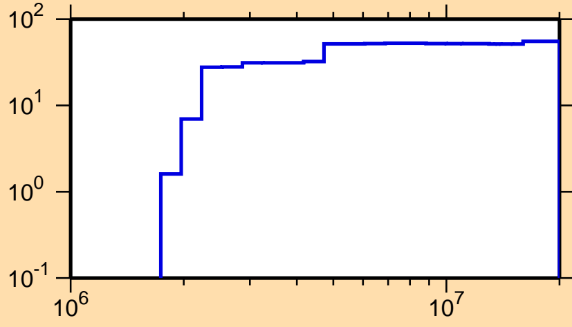
\Delta\sigma/\sigma vs. E for ^{232}\text{Pa}(n,p)
