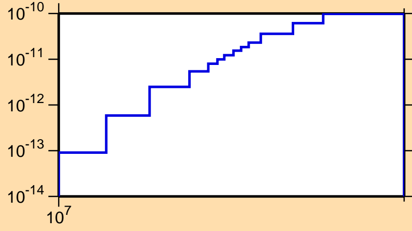
\sigma vs. E for ^{232}\text{Pa}(n,p\alpha)
