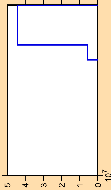
\Delta\sigma/\sigma vs. E for ^{232}\text{Pa} (mt 45)
