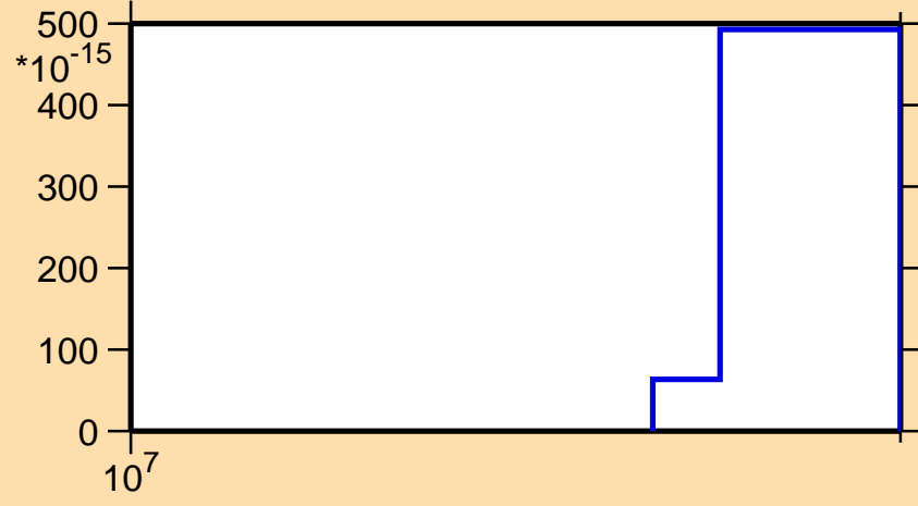
\sigma vs. E for ^{232}\text{Pa} (mt 45)
