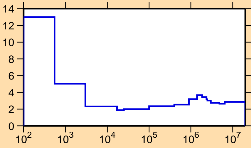
\sigma vs. E for ^{232}\text{Pa}(n,\text{nonel.})
