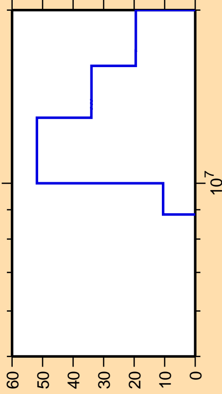
\Delta\sigma/\sigma vs. E for ^{233}\text{Pa}(n,t)
