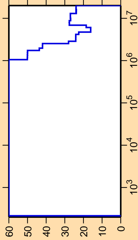
\Delta\sigma/\sigma vs. E for ^{233}\text{Pa}(n,\text{nonel.})
